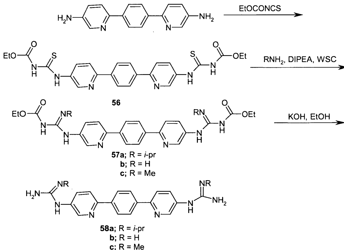
Scheme 15
