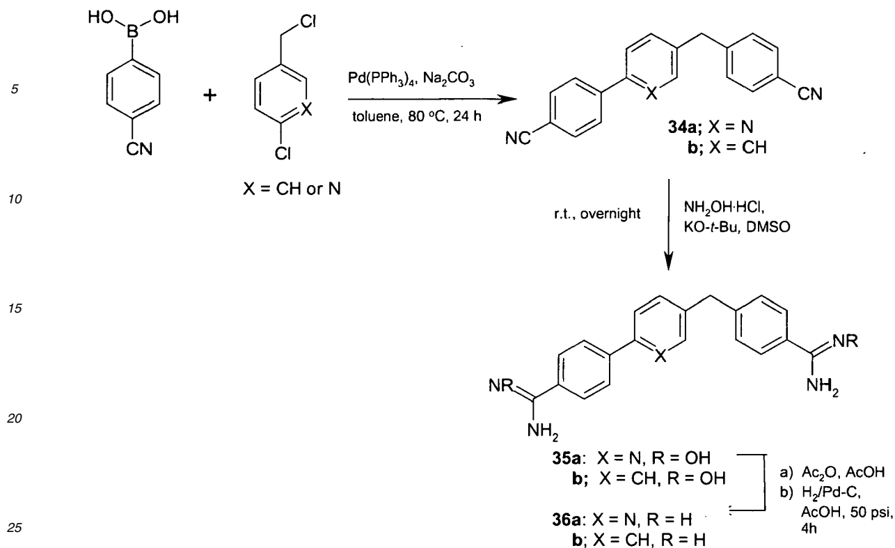
Scheme 8
