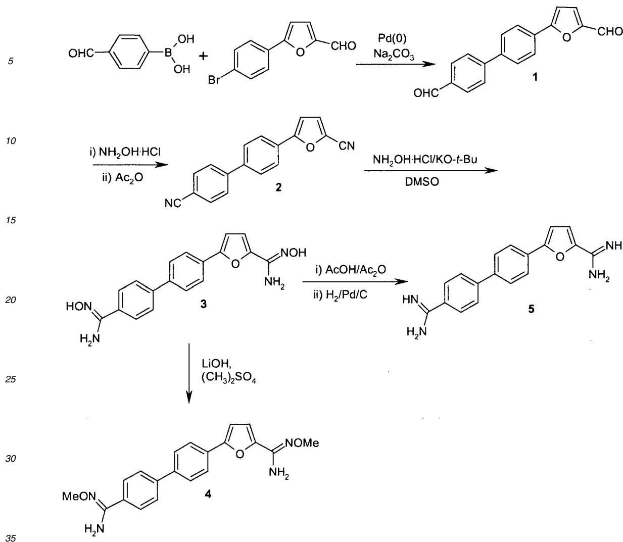
Scheme 1
