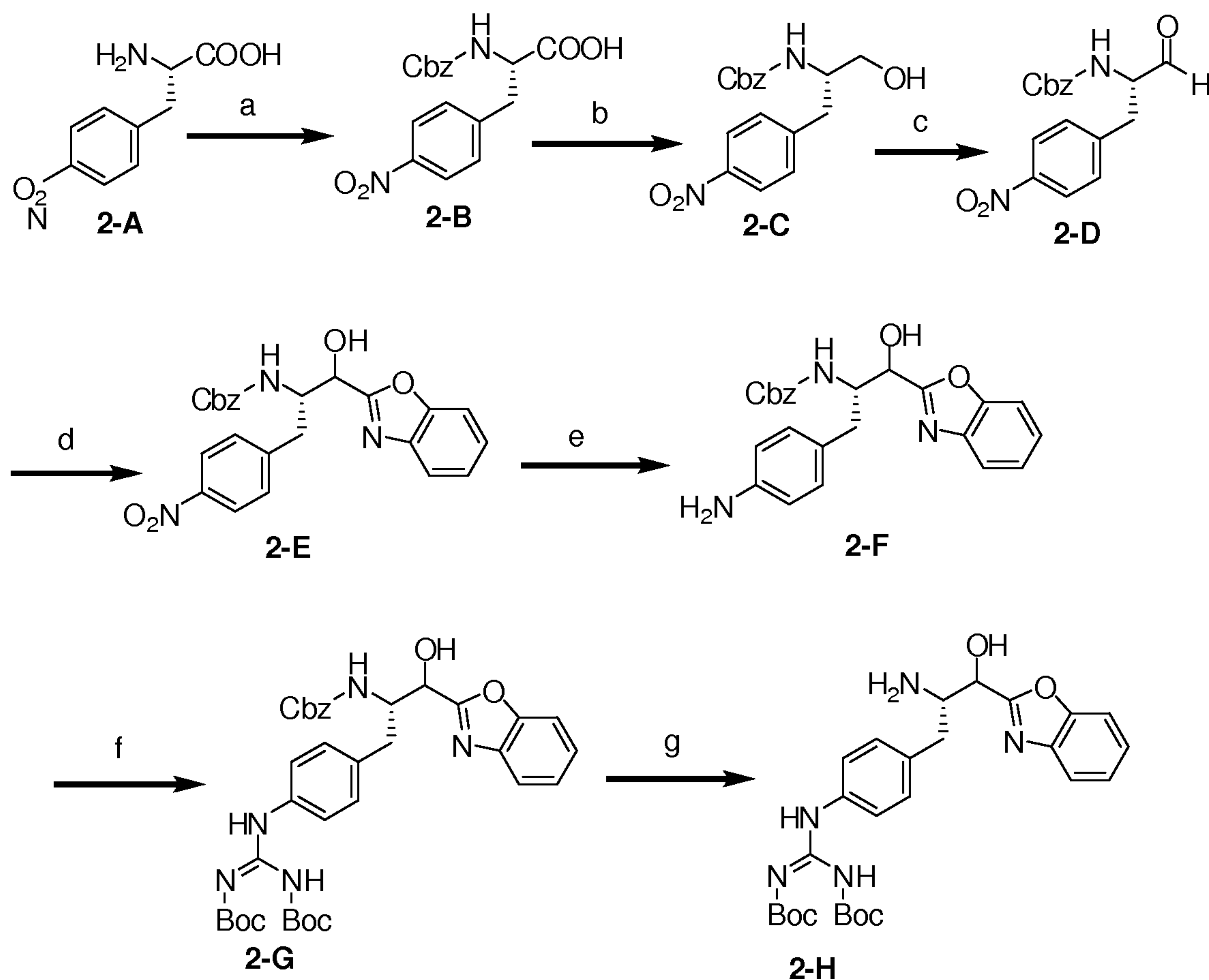
Scheme 2
