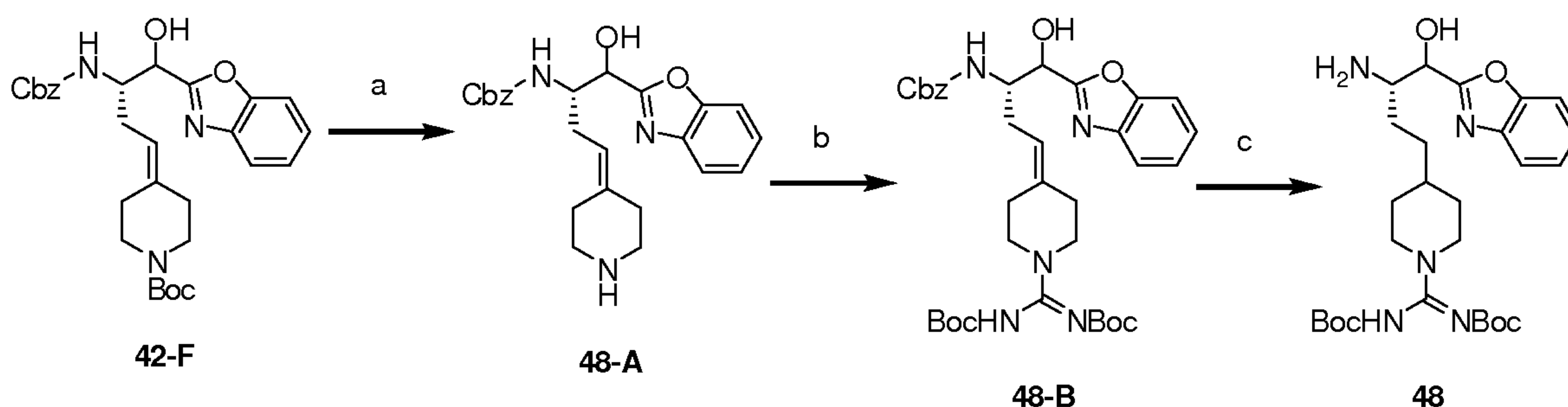
Scheme 11
