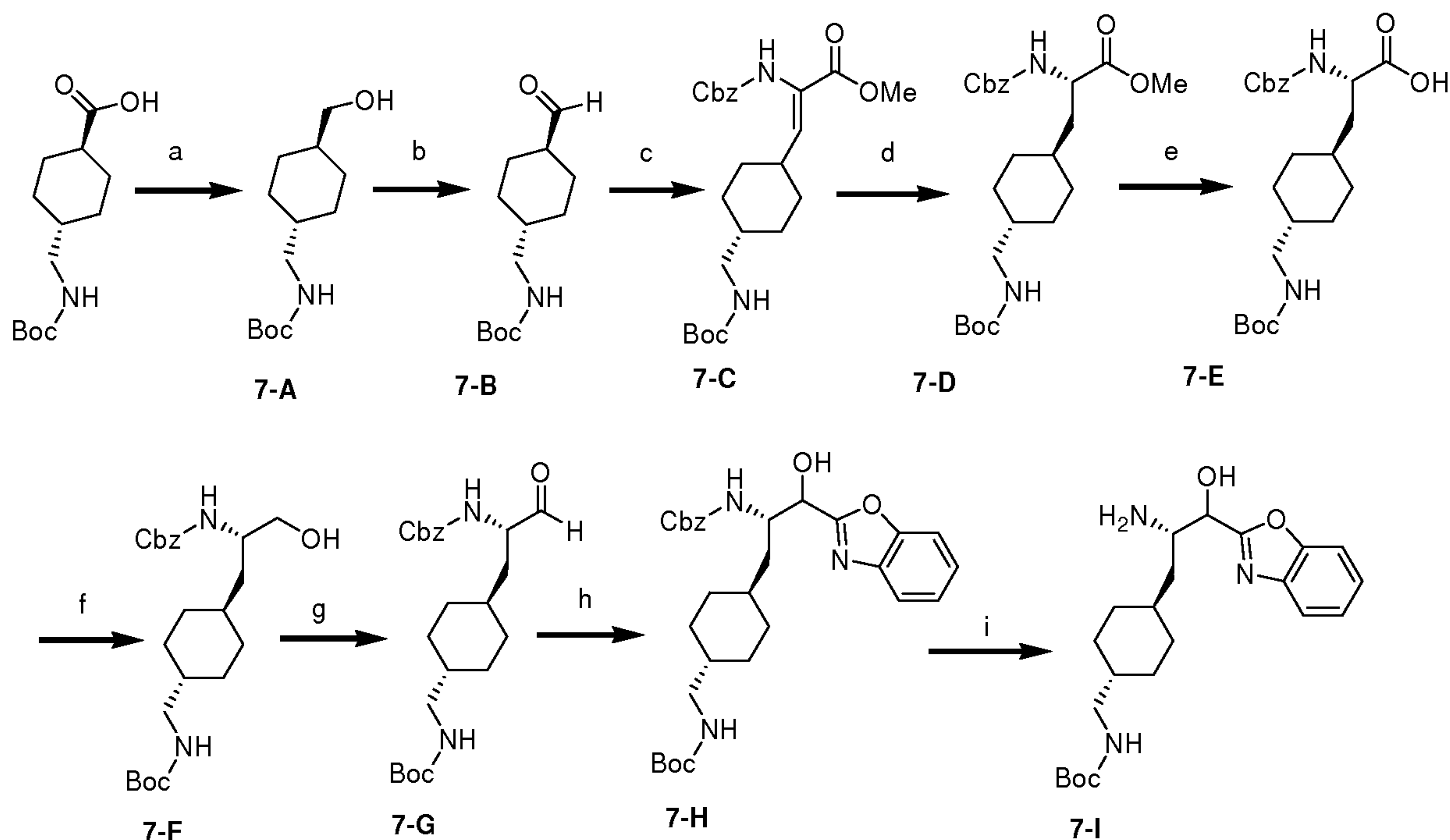
Scheme 7
