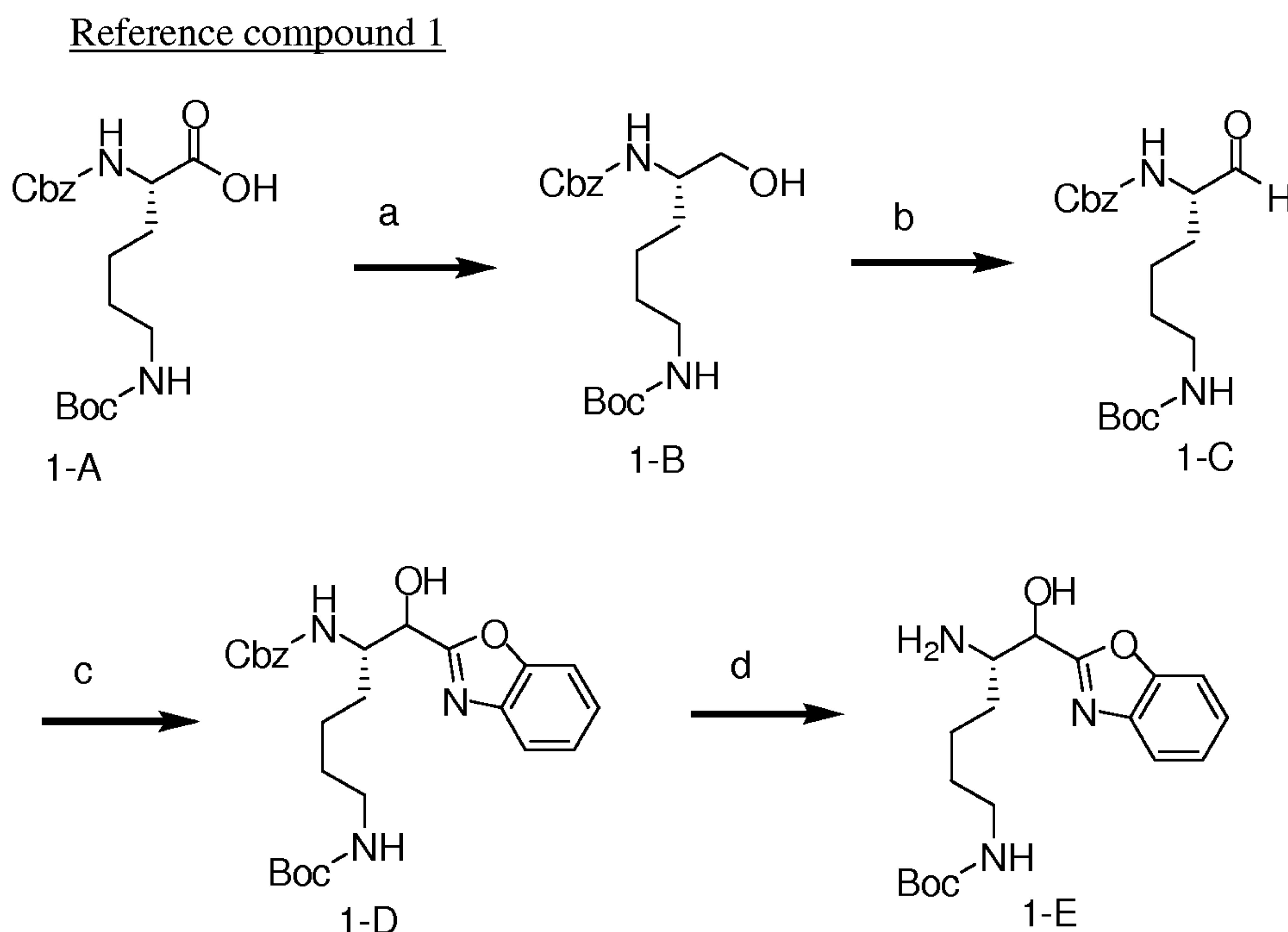
Scheme 1
