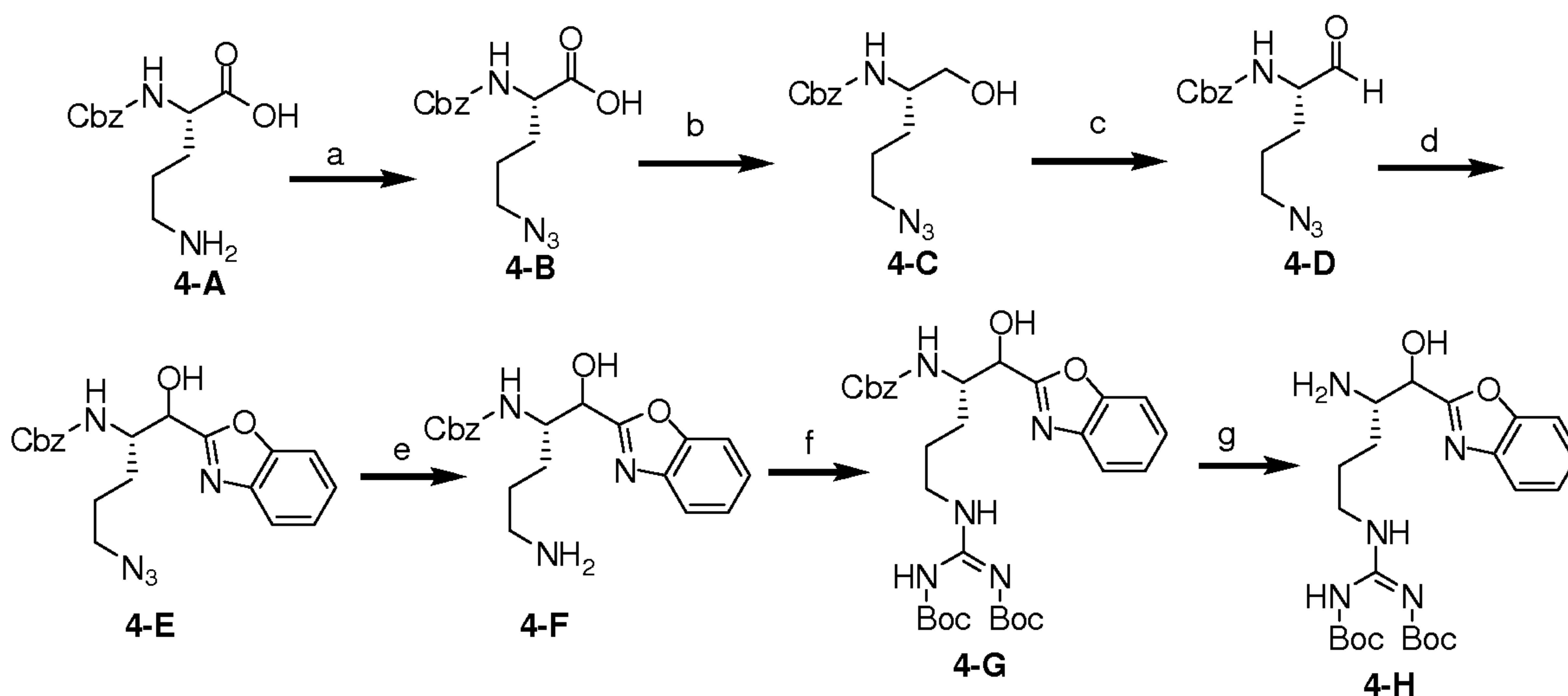
Scheme 4
