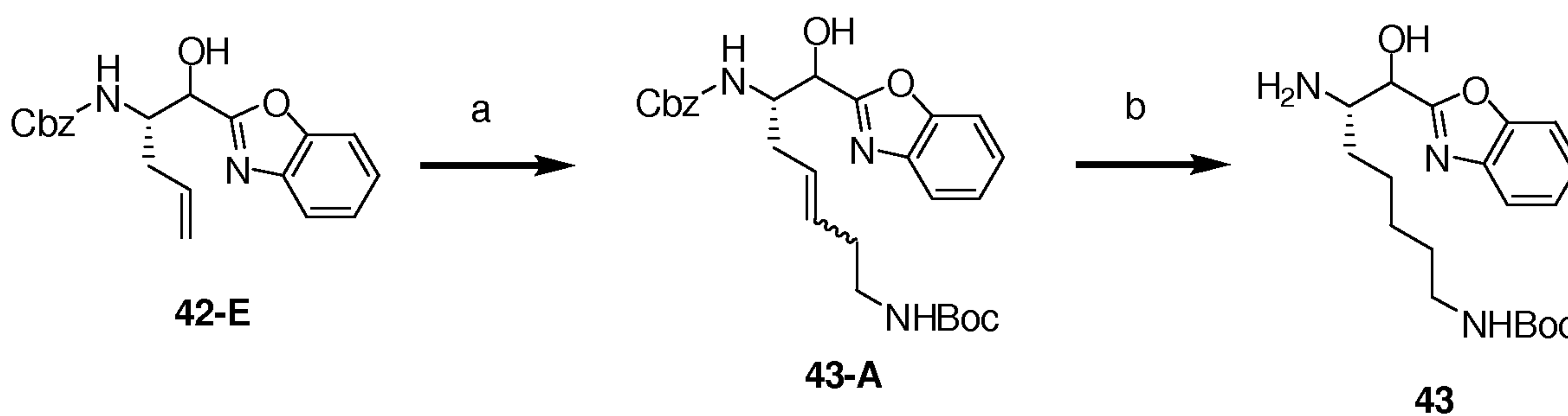
Scheme 10
