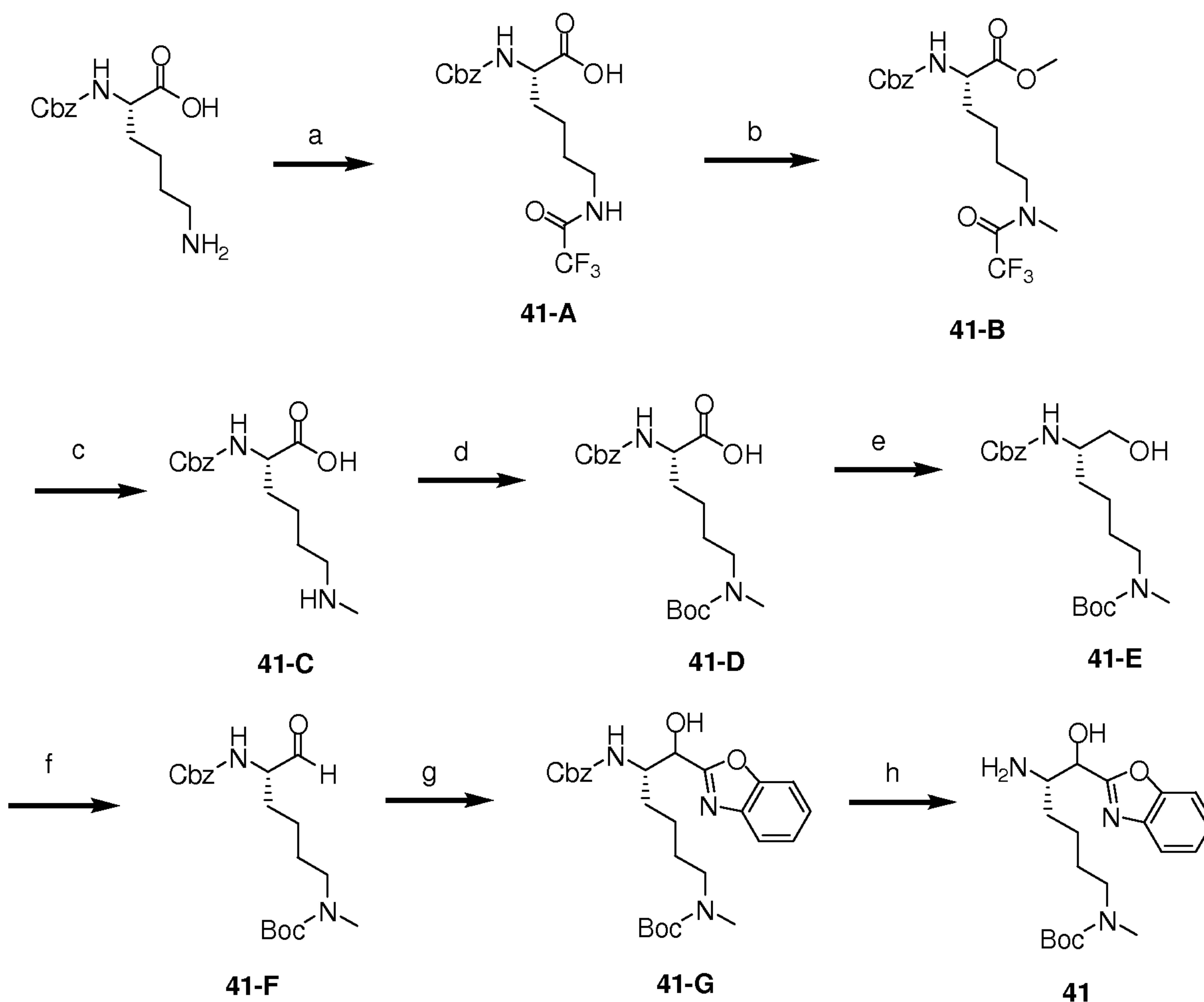
Scheme 8
