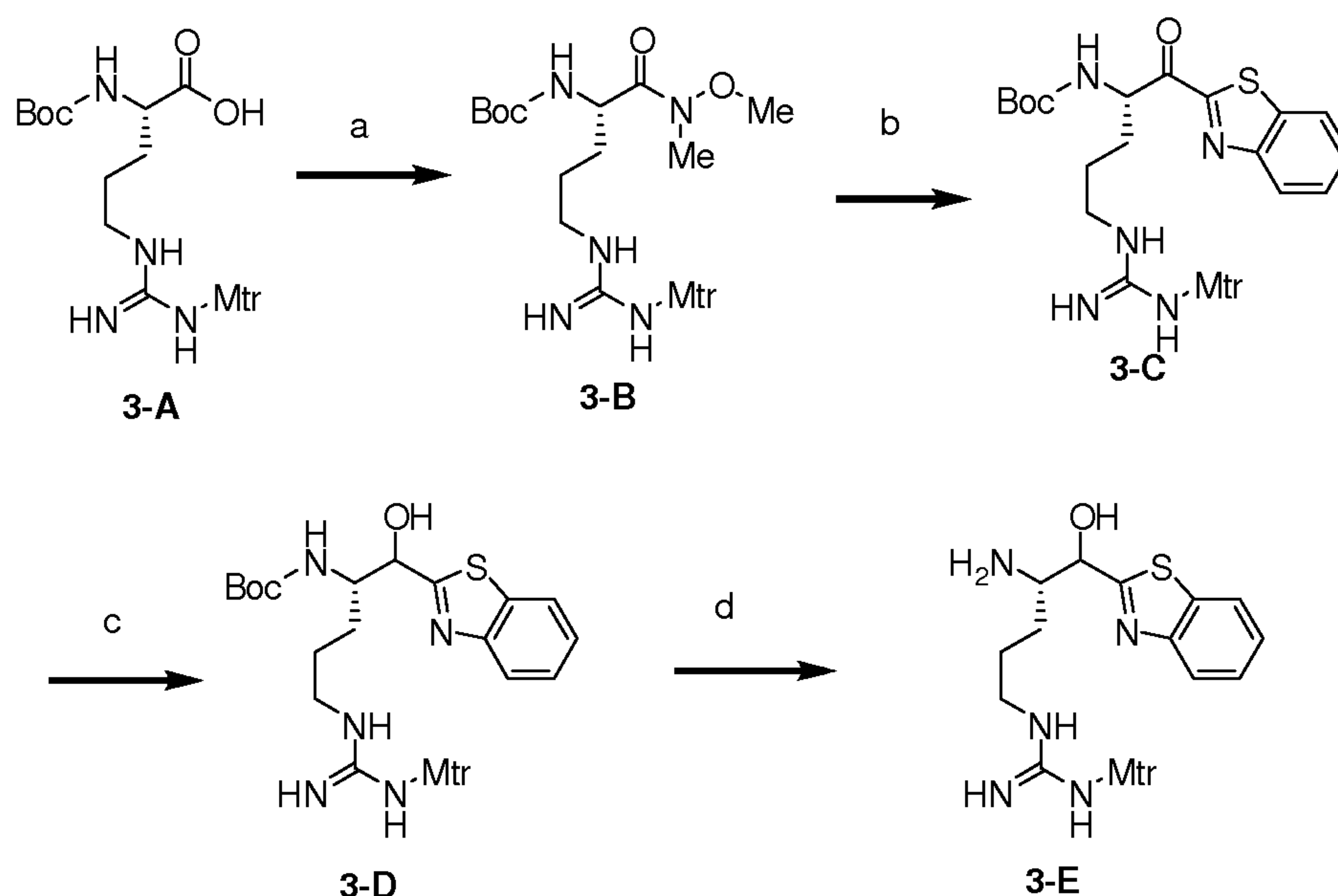
Scheme 3
