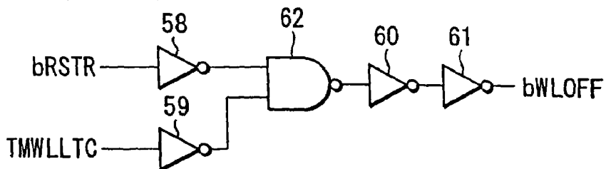
bWLOFF latch circuit
