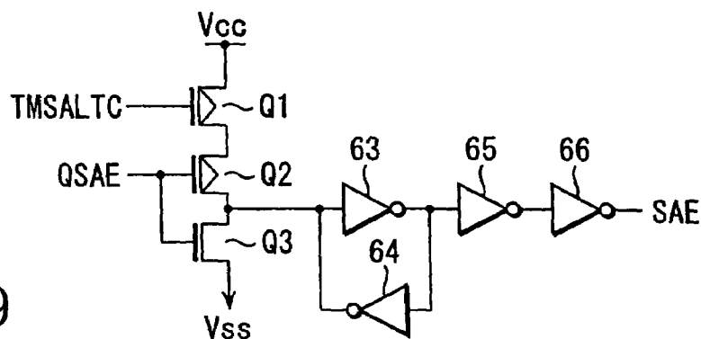
SAE latch circuit
