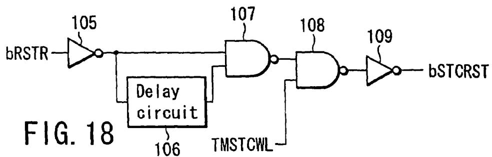
STCRST control circuit
