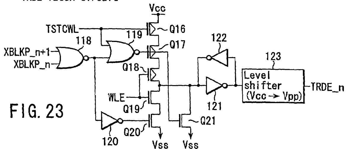
TRDE latch circuit
