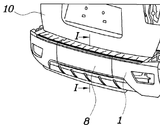
FIG. 2 (Related Art)
