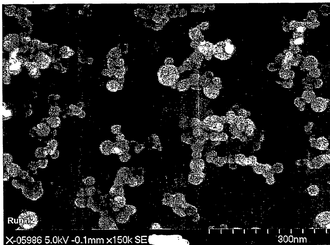
Figure 5 SEM micrograph of the \text{TiO}_2 nanoparticles produced under the condition described in Example 2
