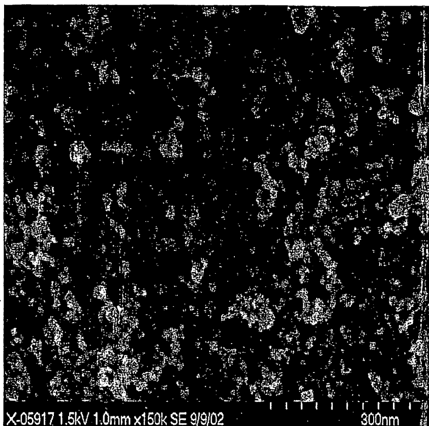
Figure 6. SEM micrograph of the \text{TiO}_2 nanoparticles produced under the condition described in Example 3
