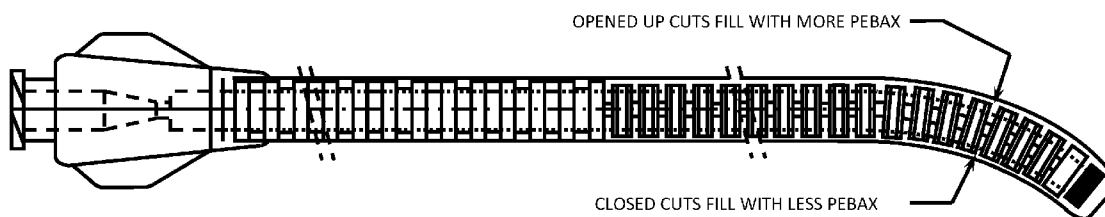
CATHETER WITH PROXIMAL CUTS FOR KINK RESISTANCE, AND SHAPE HOLDING TIP.
