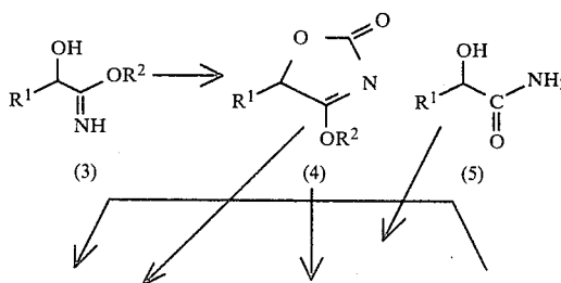
Flowsheet I Oxazolidine-2,4-dione Precursors
