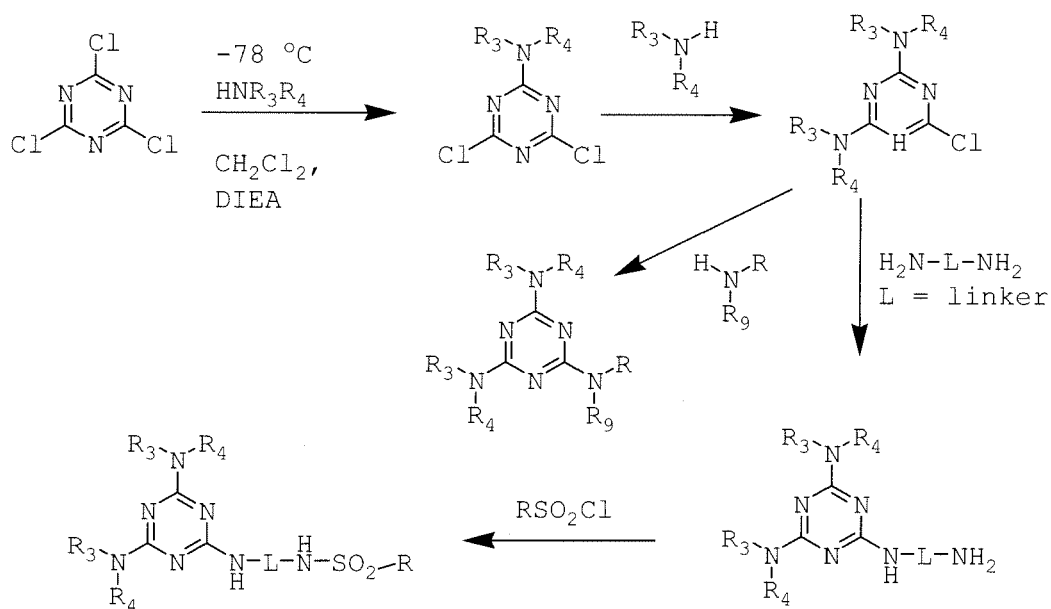
Scheme 3. Synthesis of Triaminotriazines
