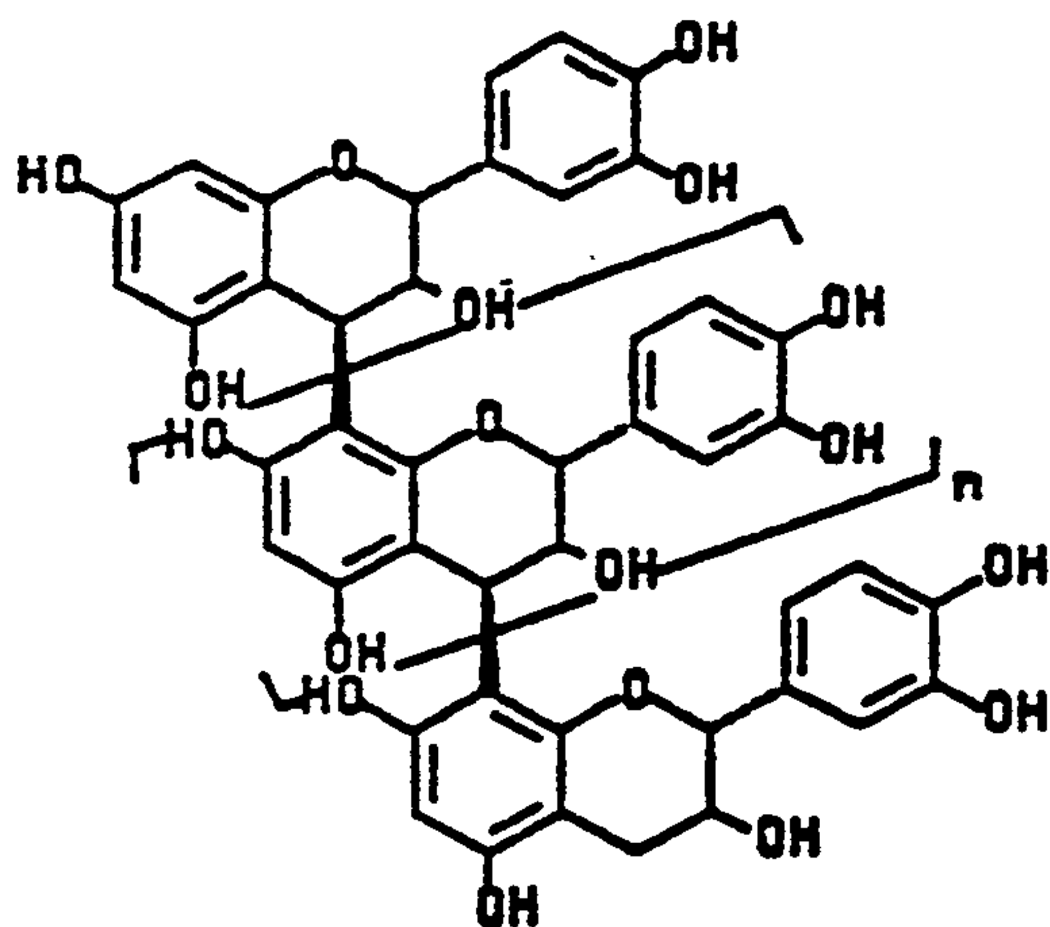
Procyanidin Oligomers n = 2 through 5
