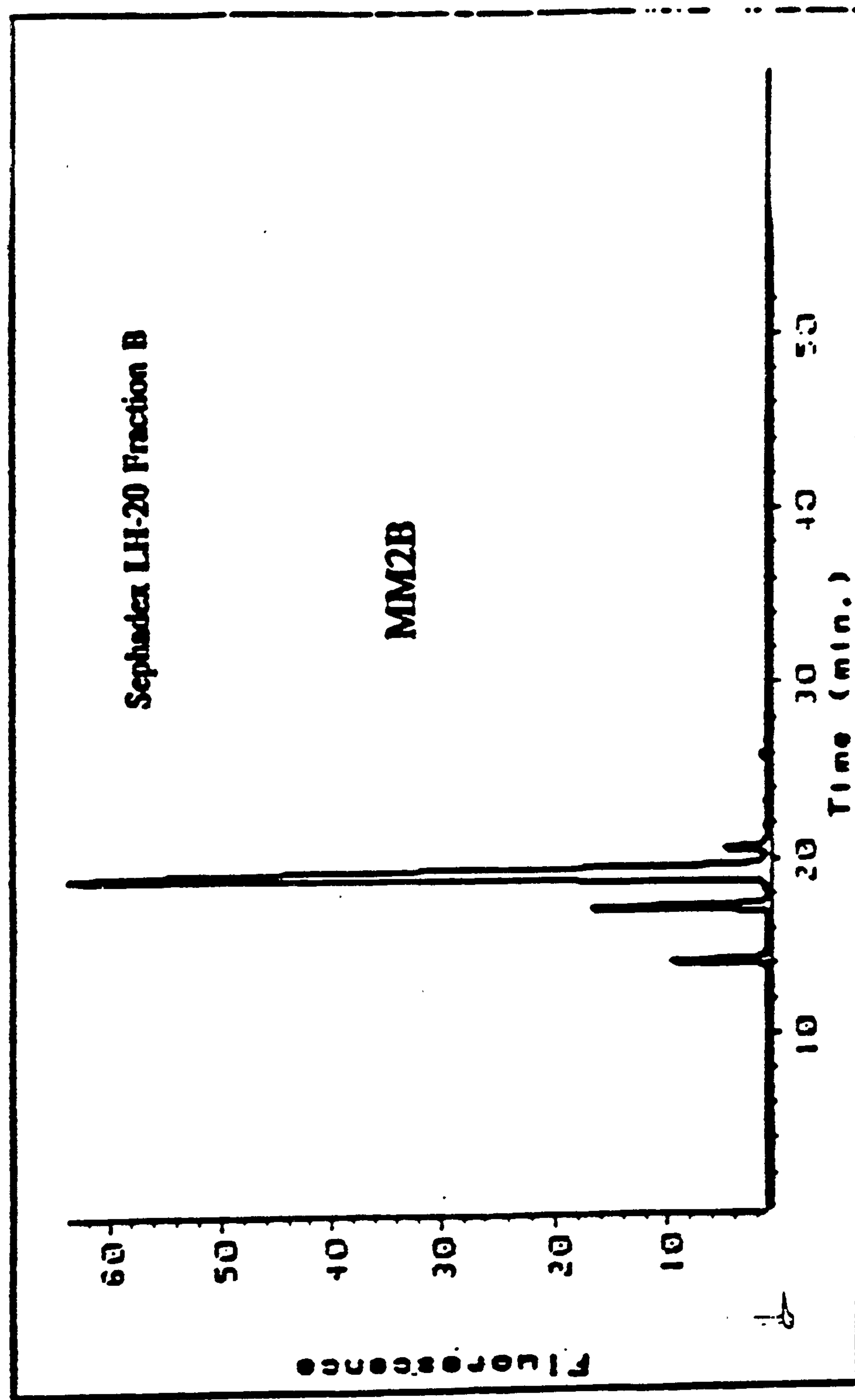
Figure 4B Representative HPLC Traces of Procyanidin Fractions
