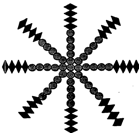
Star Copolymer
