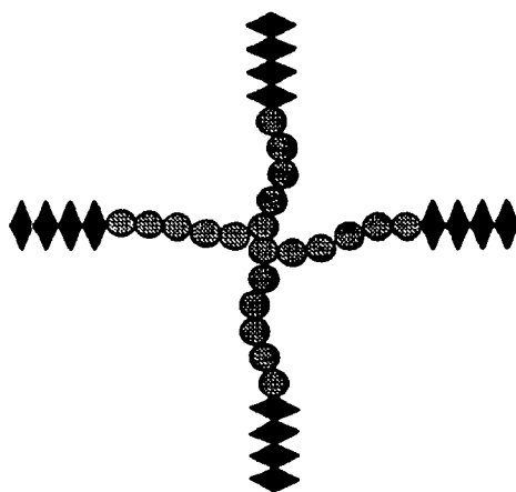
Radial Copolymer
