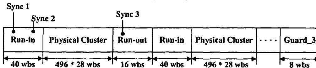
Continuously written sequence of Recording Unit Blocks
