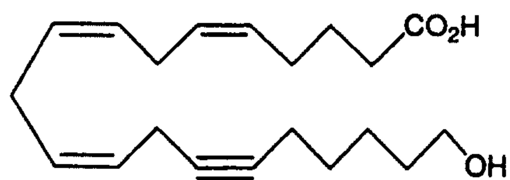
14,15-Dehydro-20-HETE (26)
