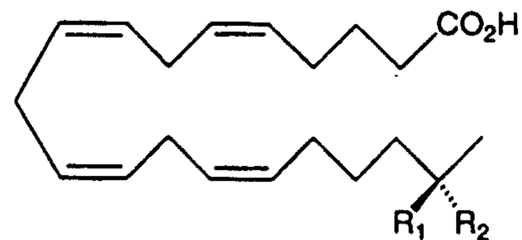
19(S)-HETE (34: R 1 = H, R 2 = OH)
