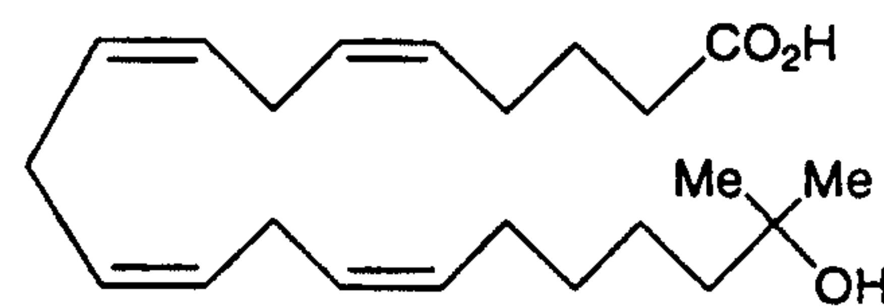
20,20-Dimethyl-20-HETE (19)
