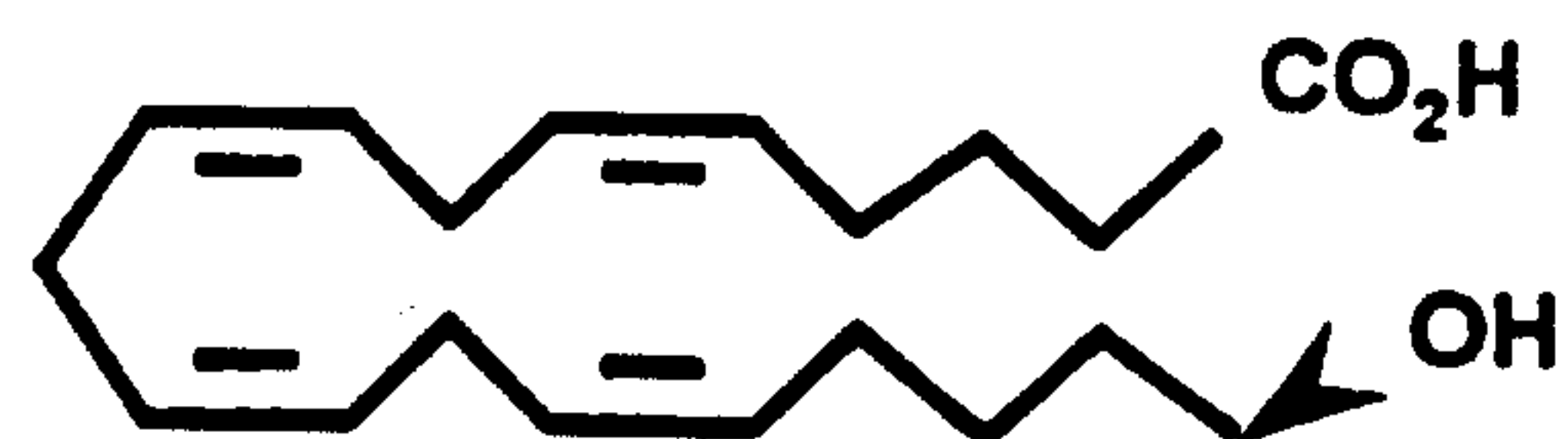
C 19 analog
