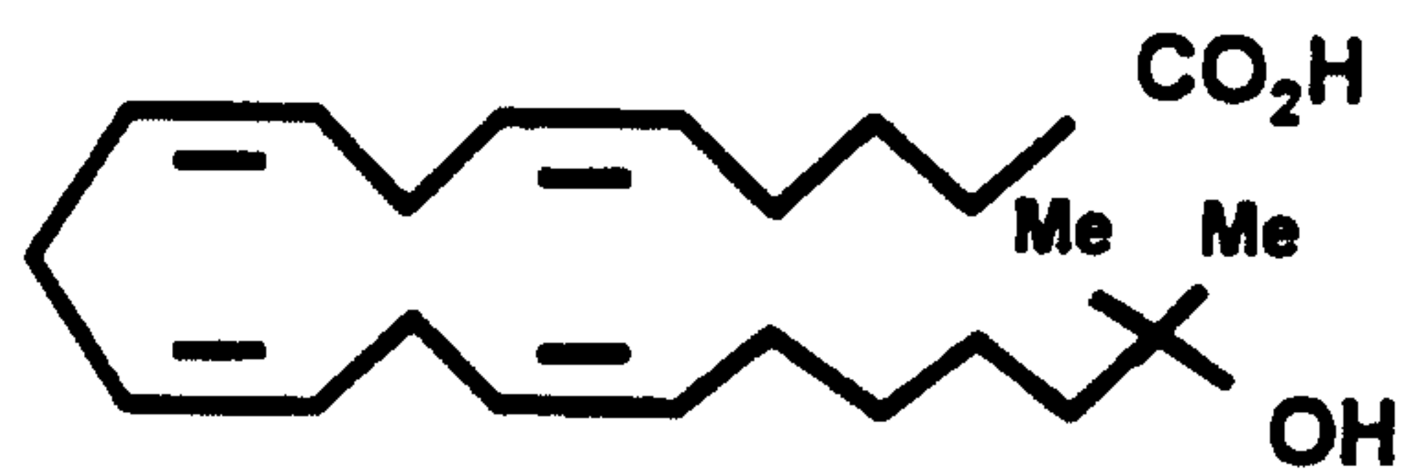
Dimethyl 20-HETE
