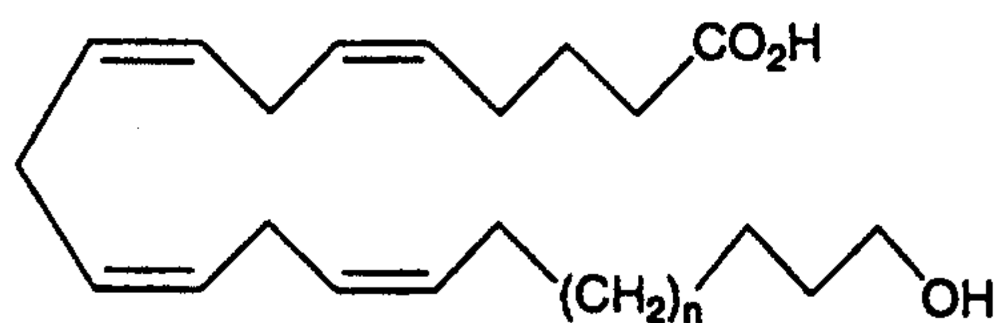
19-Hydroxynonadeca-5(Z),8(Z),11(Z),14(Z)-tetraenoic Acid (9a: n = 0)
