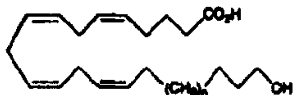
18-Hydroxynonadeca-6(Z),8(Z),11(Z),14(Z)-tetraenoic Acid (8a; n = 0)
