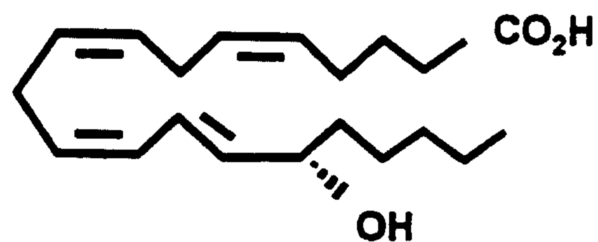
15(S)-HETE
