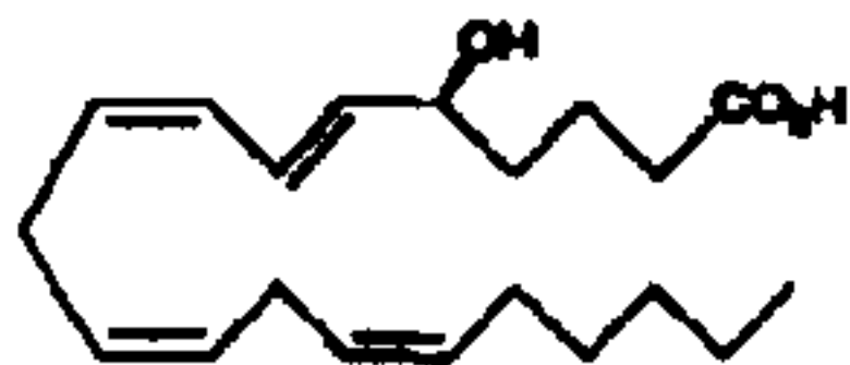
8(S)-HETE
