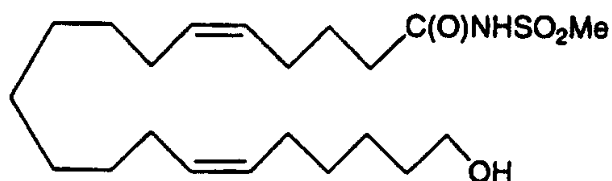
N-Methylsulfonyl-20-Hydroxyeicosa-5(Z),14(Z)-dienamide
