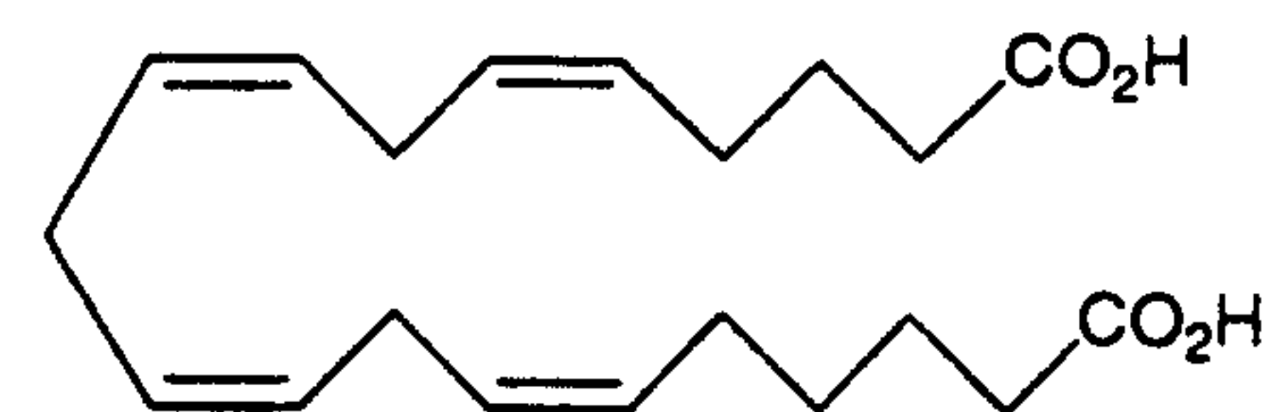
Eicosatetraen-1,20-dioic Acid
