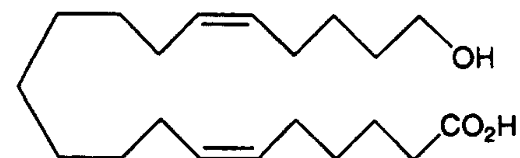
20-Hydroxyeicosa-6(Z),15(Z)-dienoic Acid (54)
