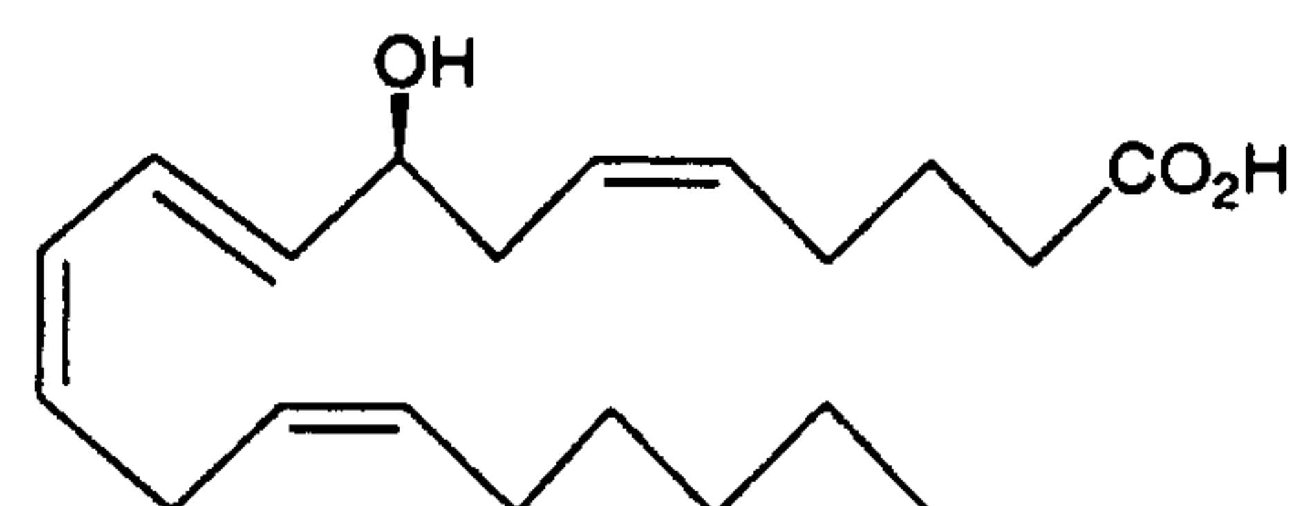
8(S)-HETE
