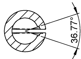
1172 SECTION B-B
