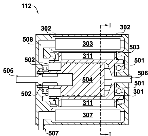
SECTION II-II
