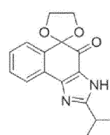
Compound 190
