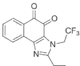
Compound 39
