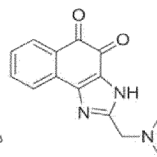
Compound 58
