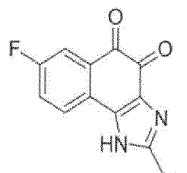
Compound 26
