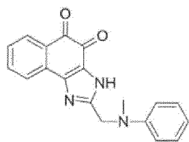
Compound 50
