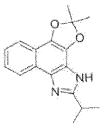
Compound 185
