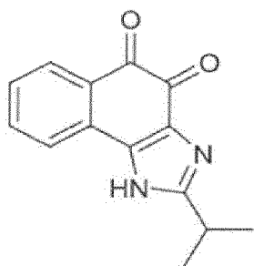
Compound 1
