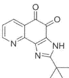
Compound 27
