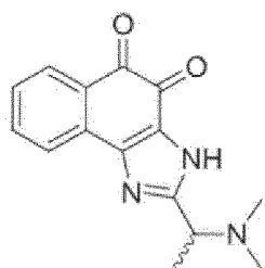
Compound 59
