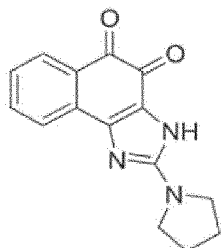
Compound 62
