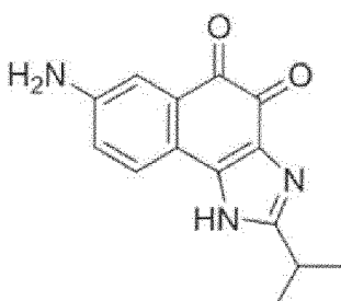
Compound 17
