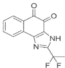
Compound 81
