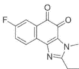
Compound 40
