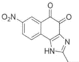
Compound 24
