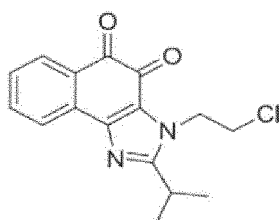
Compound 63
