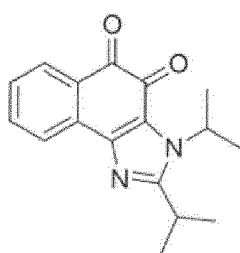
Compound 84
