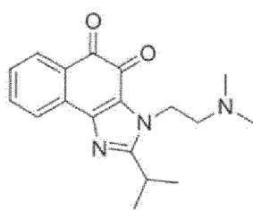
Compound 71
