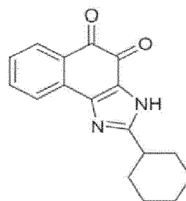
Compound 6
