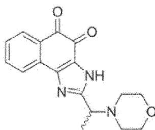
Compound 60
