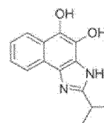
Compound 175
