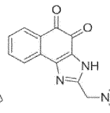
Compound 58
