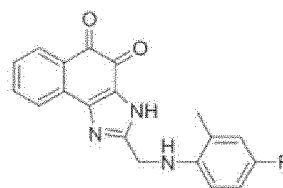
Compound 52
