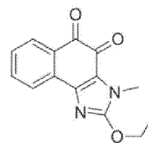
Compound 73
