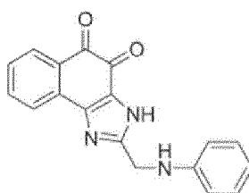
Compound 48
