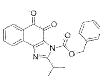
Compound 31
