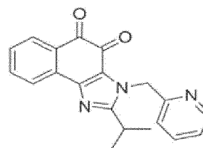
Compound 83
