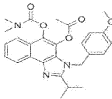
[Compound 181]
