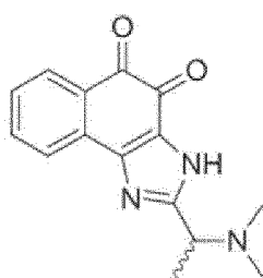
Compound 59
