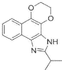
Compound 189
