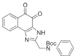
Compound 47
