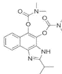
Compound 183
