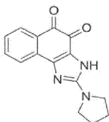
Compound 62
