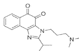
Compound 55
