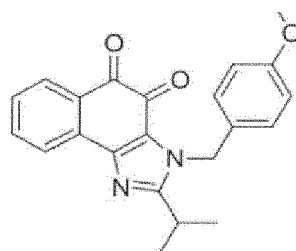
Compound 30
