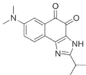
Compound 23
