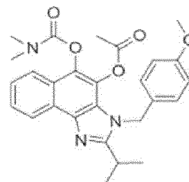
Compound 181
