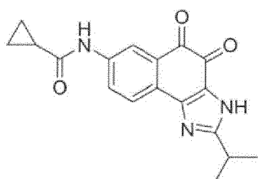
Compound 19
