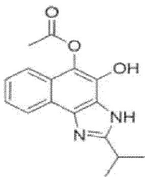
[Compound 176]
