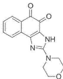
Compound 66
