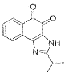
Compound 96
