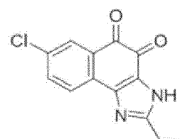
Compound 44
