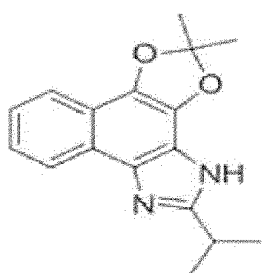
[Compound 185]
