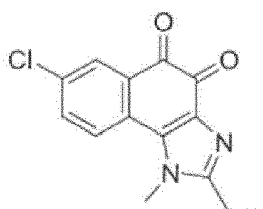
Compound 43
