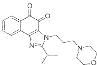
Compound 56
