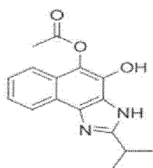
Compound 176
