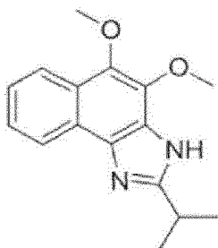
Compound 188
