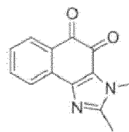
Compound 95
