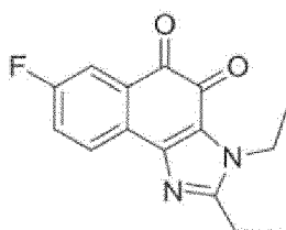
Compound 87
