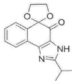
Compound 190
