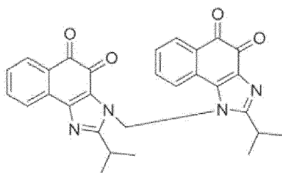
Compound 68
