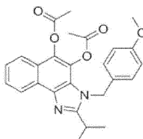
Compound 180
