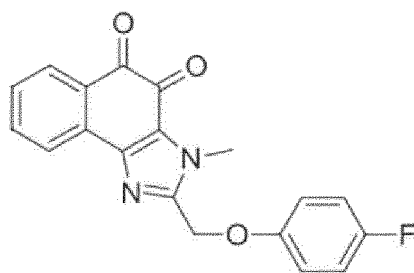
Compound 79
