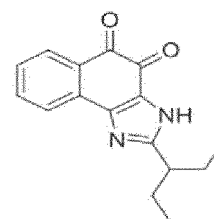
Compound 76
