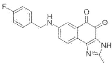
Compound 46
