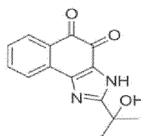
Compound 75
