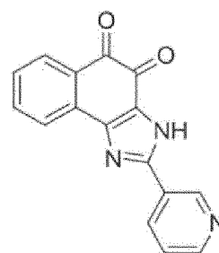
Compound 86
