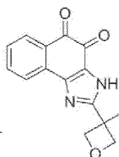
Compound 98
