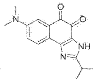
Compound 23
