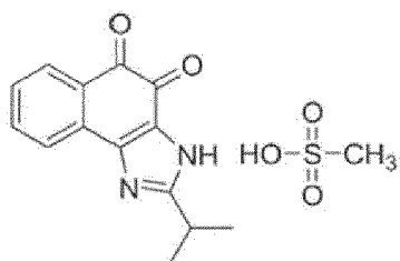
Compound 96
