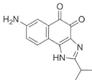
Compound 17
