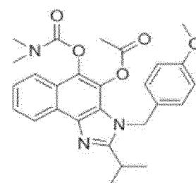
Compound 181
