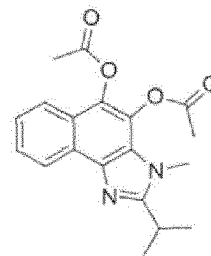
Compound 184
