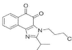
Compound 54
