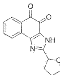
Compound 72
