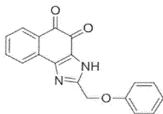
Compound 77
