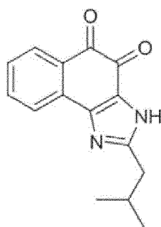
Compound 8
