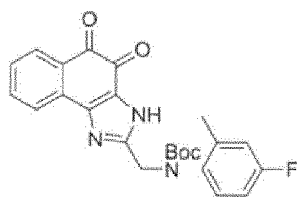
Compound 51
