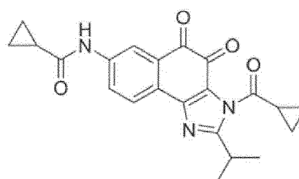
Compound 20
