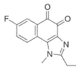
Compound 41
