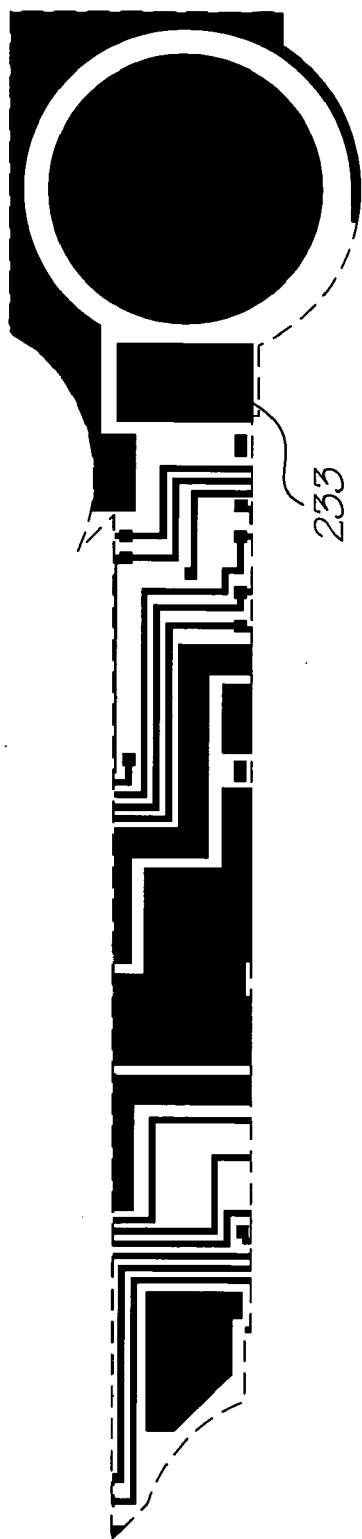
Metal 2 mask
