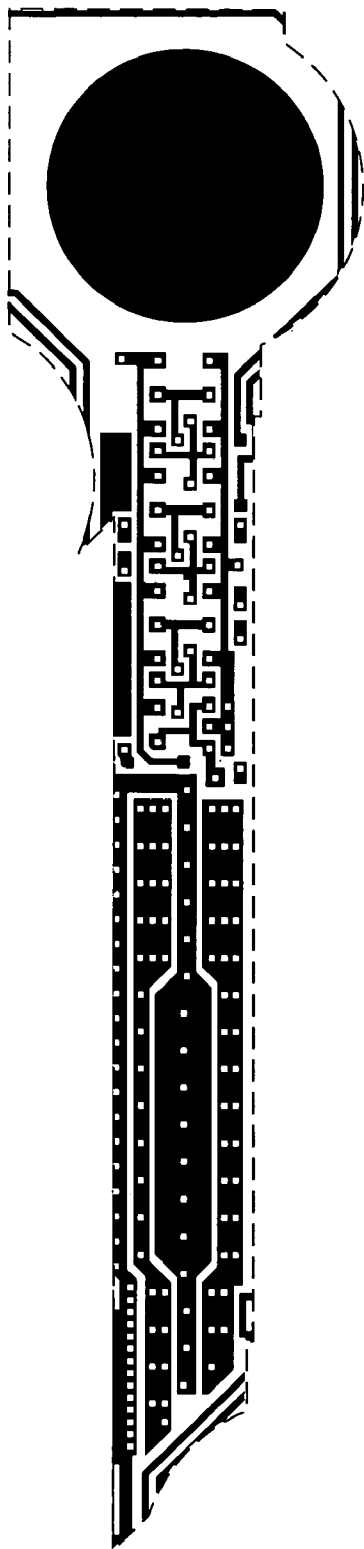
Metal 1 mask
