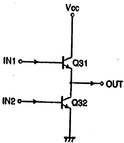
Fig. 4 (PRIOR ART)
