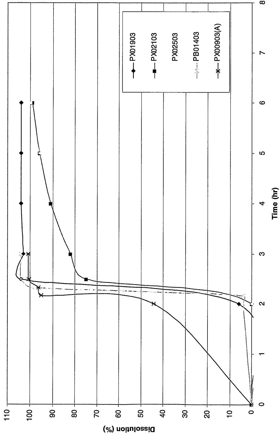
Dissolution of Baclofen Controlled-release Capsules, 20 mg SGF switchover to SIF at t.p.=2 hr, USP basket/75 rpm
