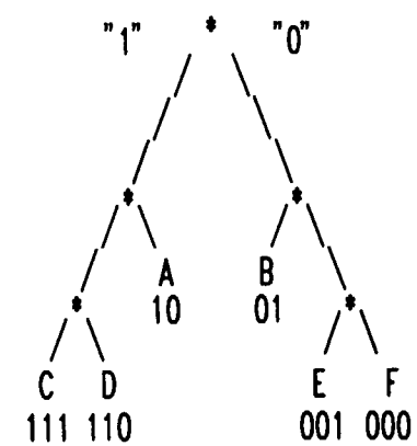
(a) NON-CANONICAL HUFFMAN CODING TREE
