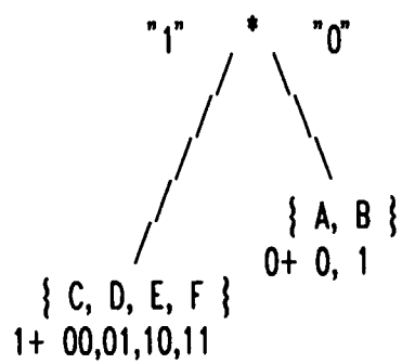
(c) CODE (LEAF) FUSION
