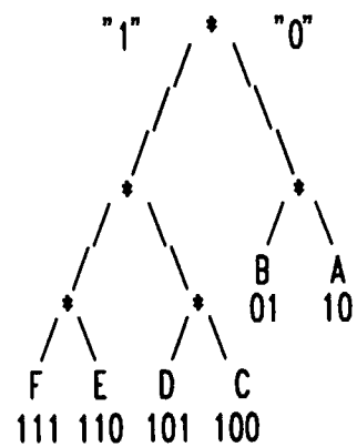
(b) CANONICAL HUFFMAN CODING TREE
