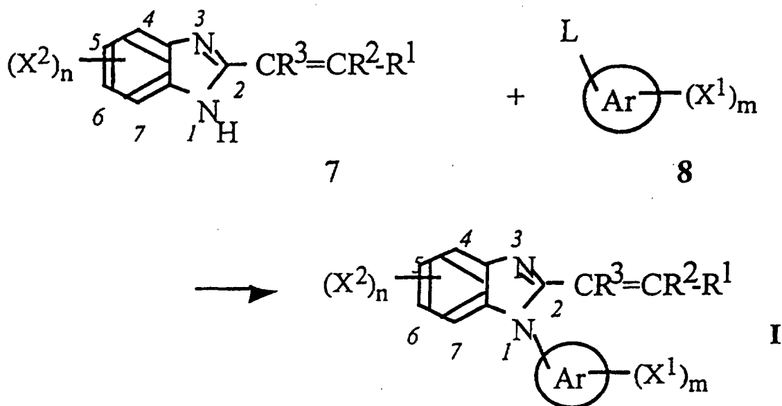
Scheme D
