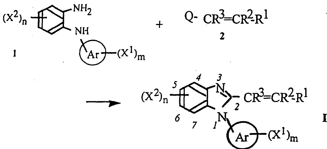
Scheme A
