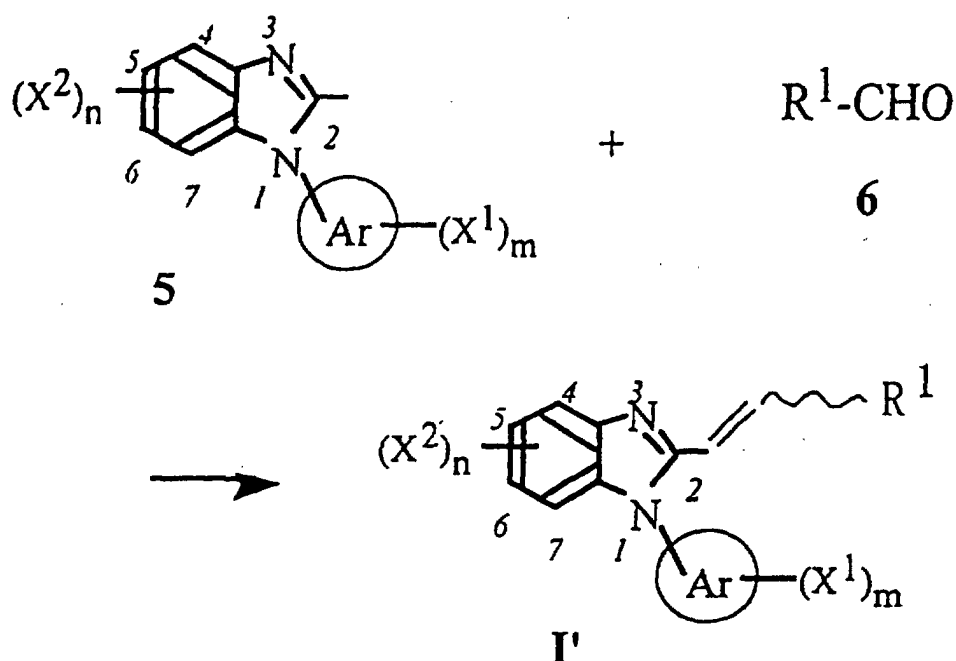
Scheme C
