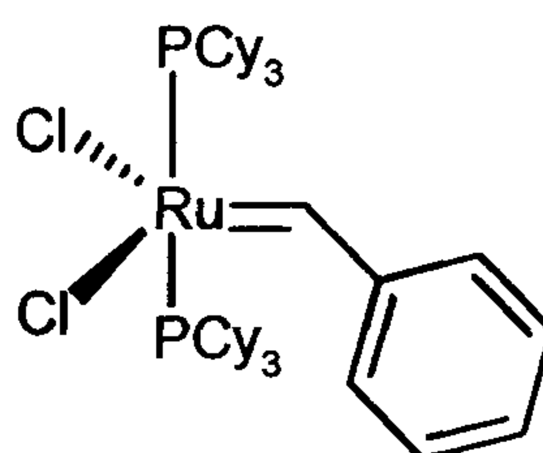
Grubbs (I) catalyst
