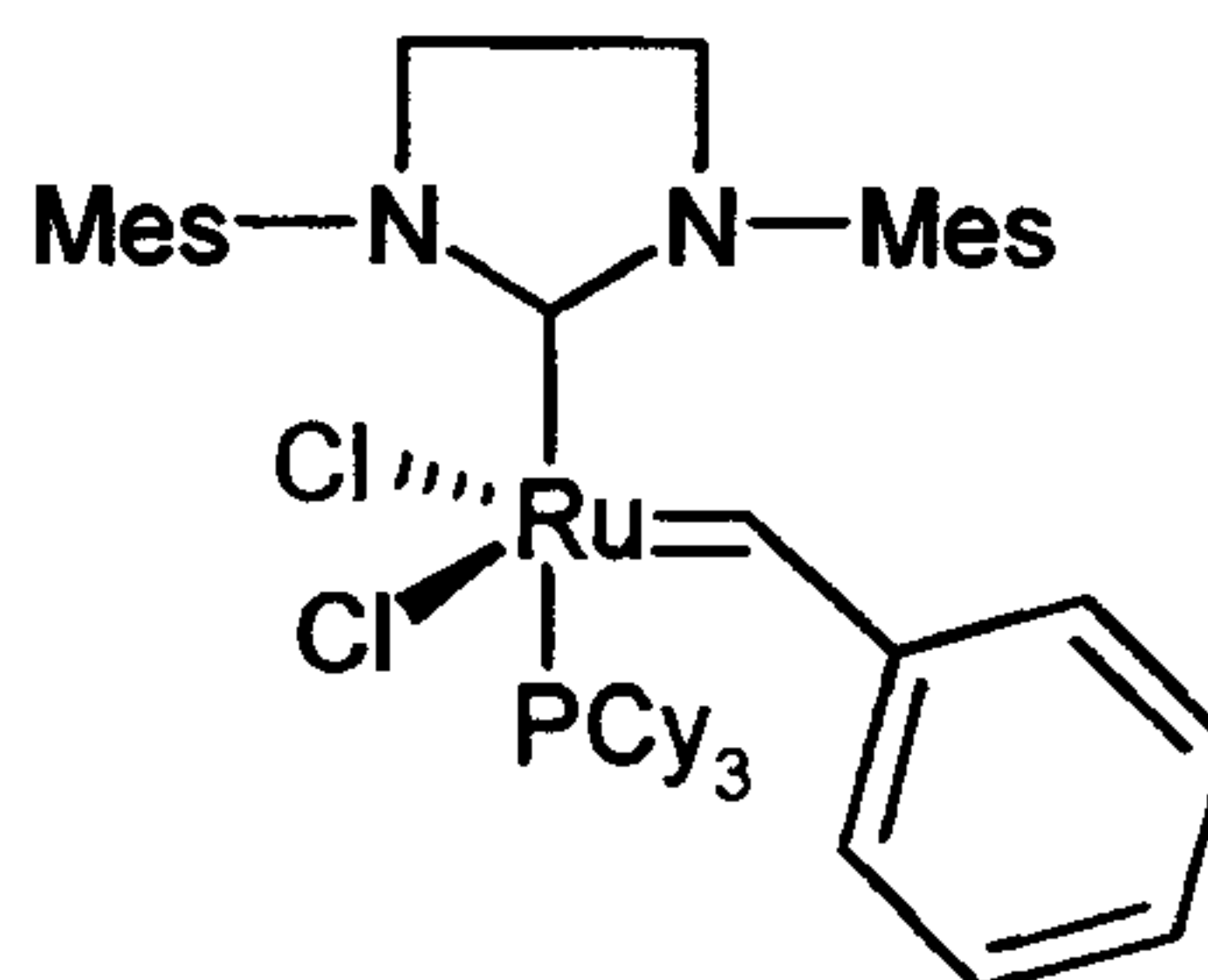
Grubbs (II) catalyst
