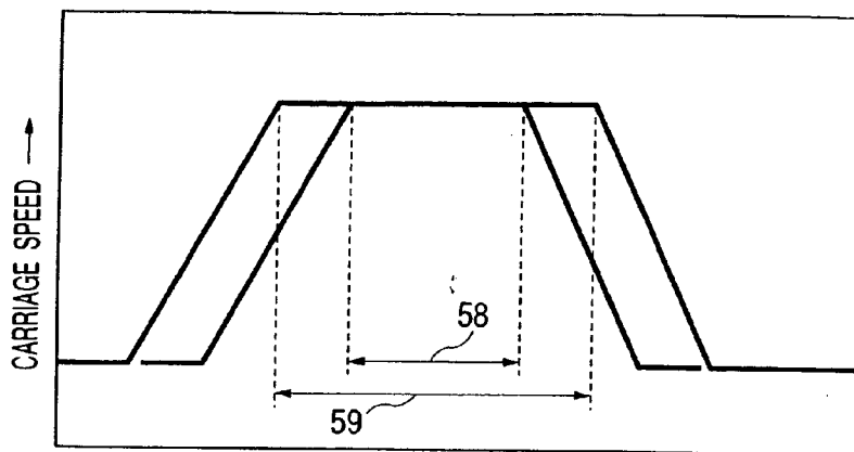
OPERATION RANGE OF CARRIAGE DURING STEP-PRINTING OPERATION
