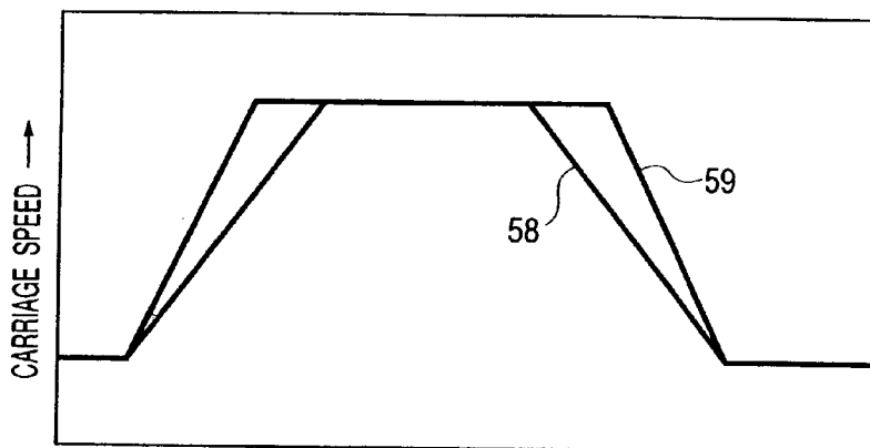
OPERATION RANGE OF CARRIAGE DURING STEP-PRINTING OPERATION
