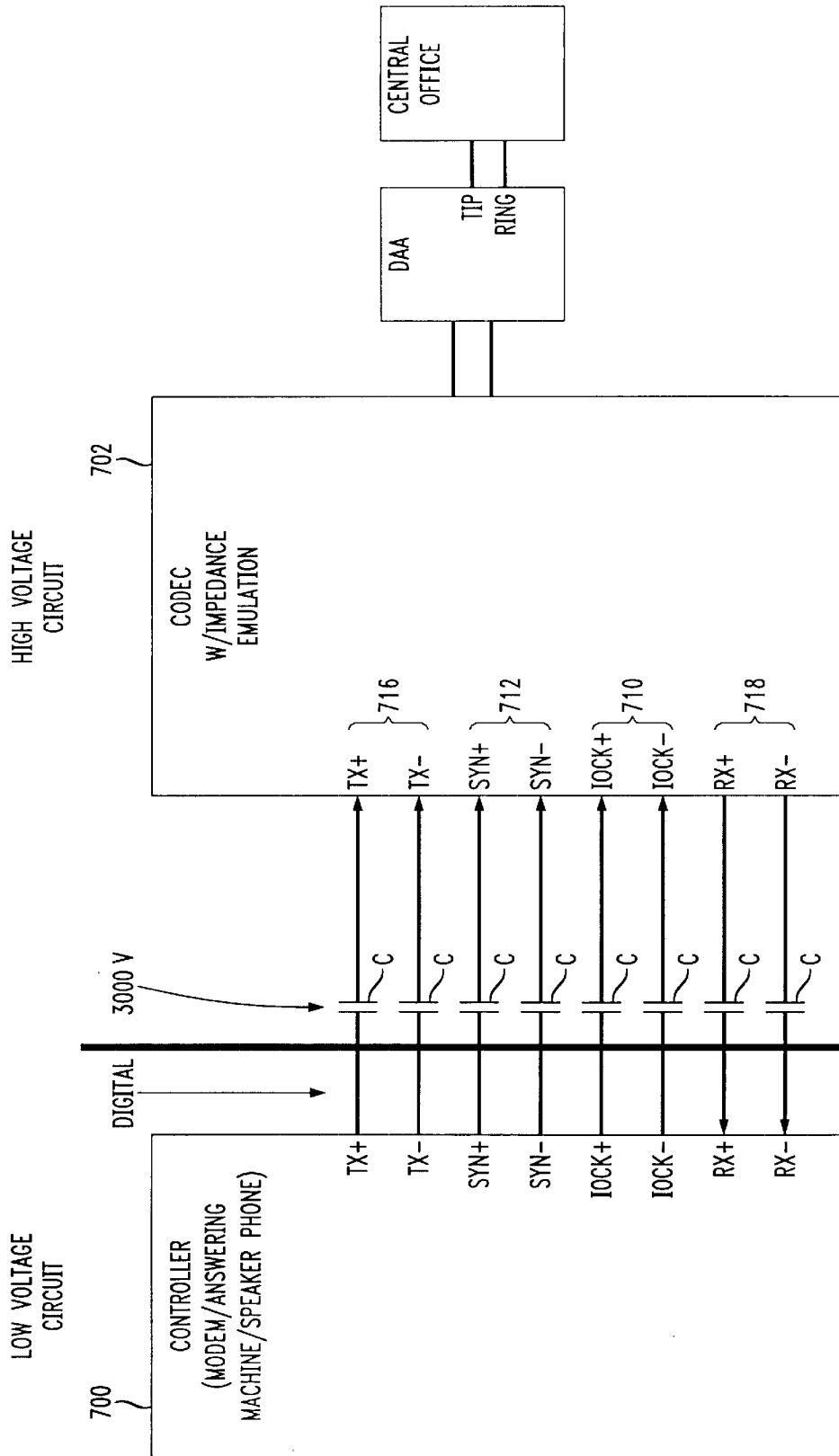
FIG. 7 PRIOR ART
