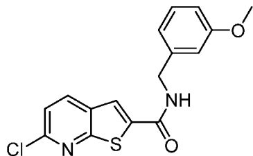
6-chloro-N-(3-methoxybenzyl)thieno[2,3-b]pyridine-2-carboxamide
