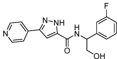
Compound 14
