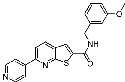
Compound 39
