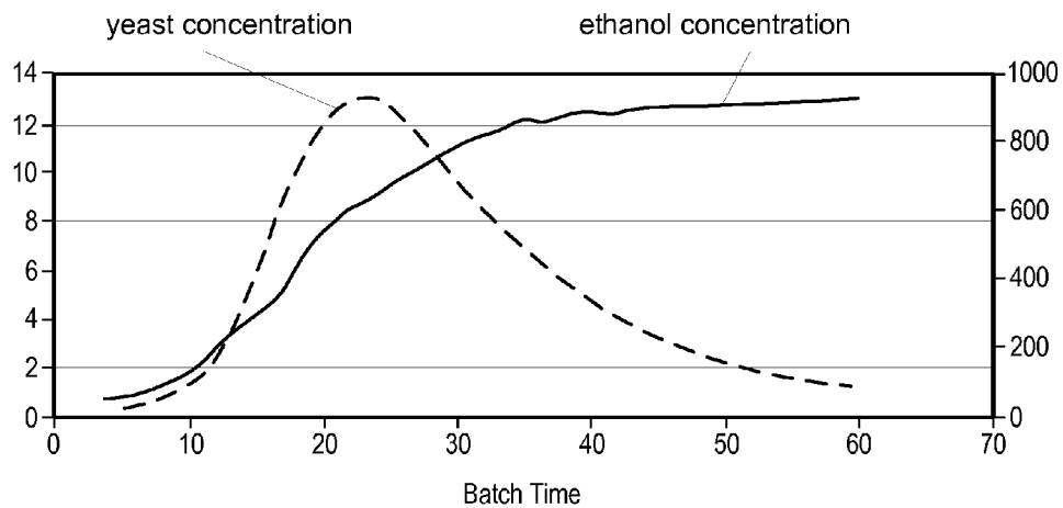
FIG. 3 (PRIOR ART)
