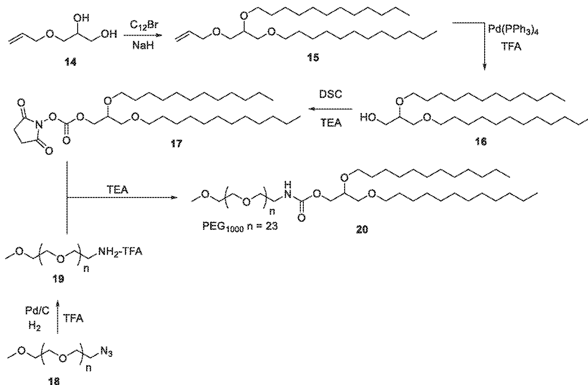
Scheme 3: Synthesis of MethoxyPEG 1000 -DiLaurylGlycerol (DLG)
