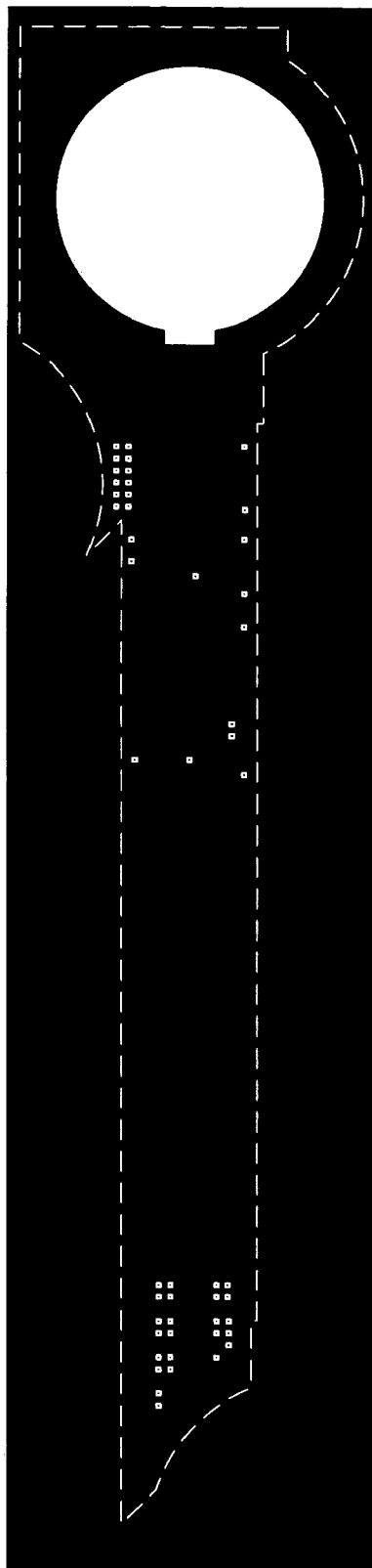
Via 1 mask
