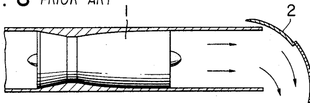
FIG. 8 PRIOR ART
