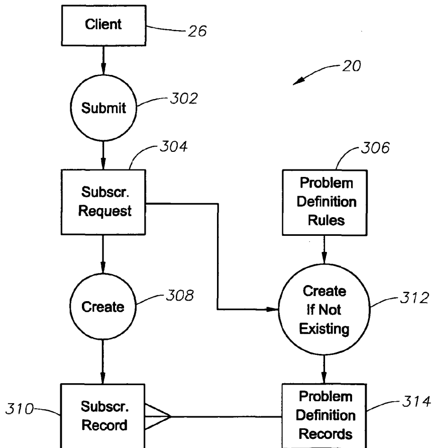
Fig. 3 Subscription Entry
