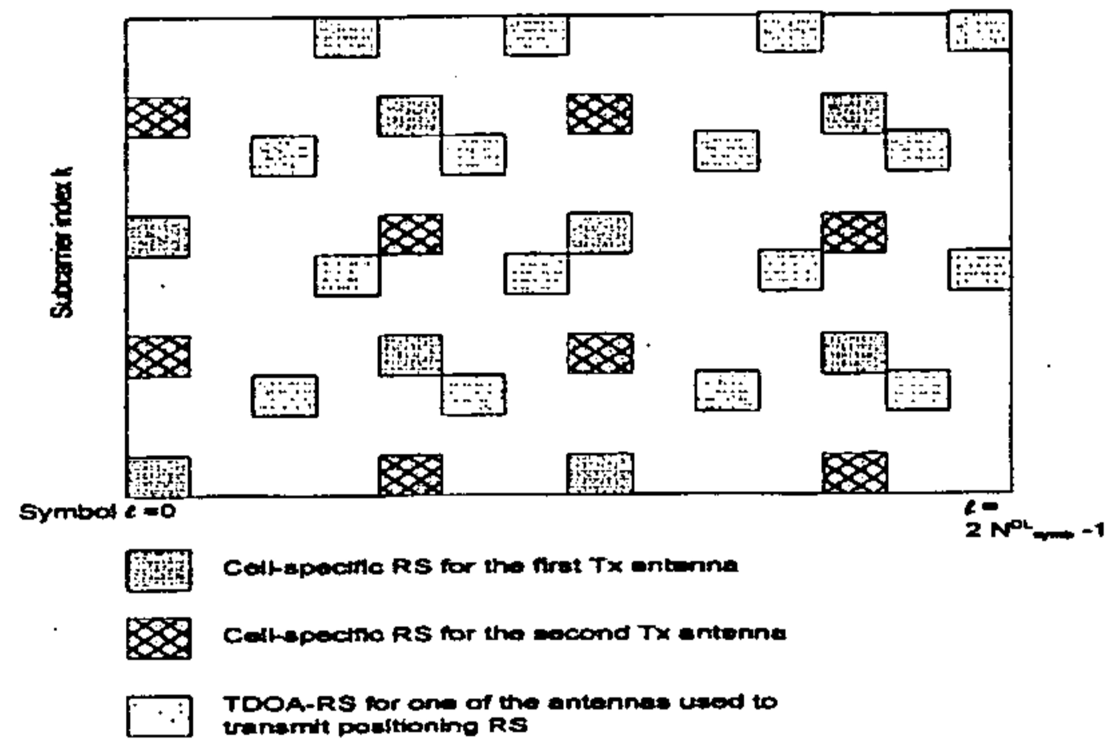
TDOA-RS with reuse 6 pattern, for deployments with more than 2-Tx antennas, but only 1 antenna port is used for the transmission of positioning RS
