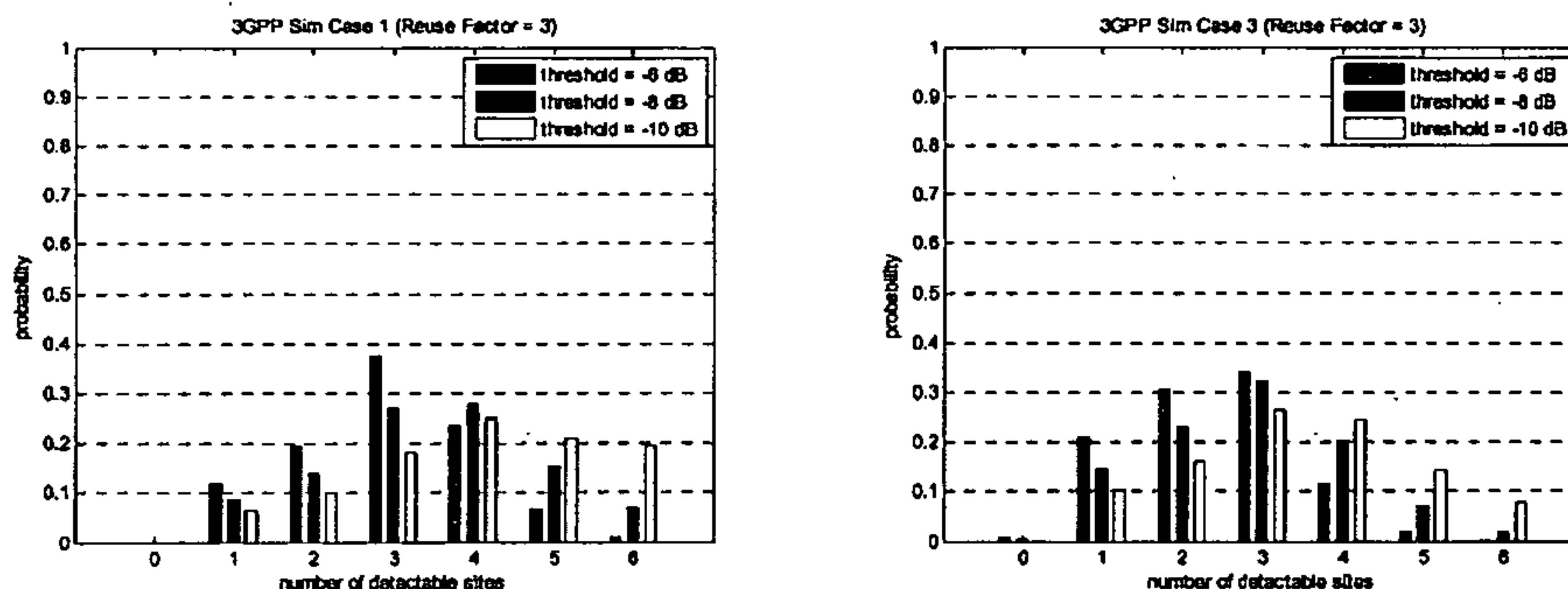
Figure 5: Distributions of number of detectable sites (Reuse Factor = 3).
