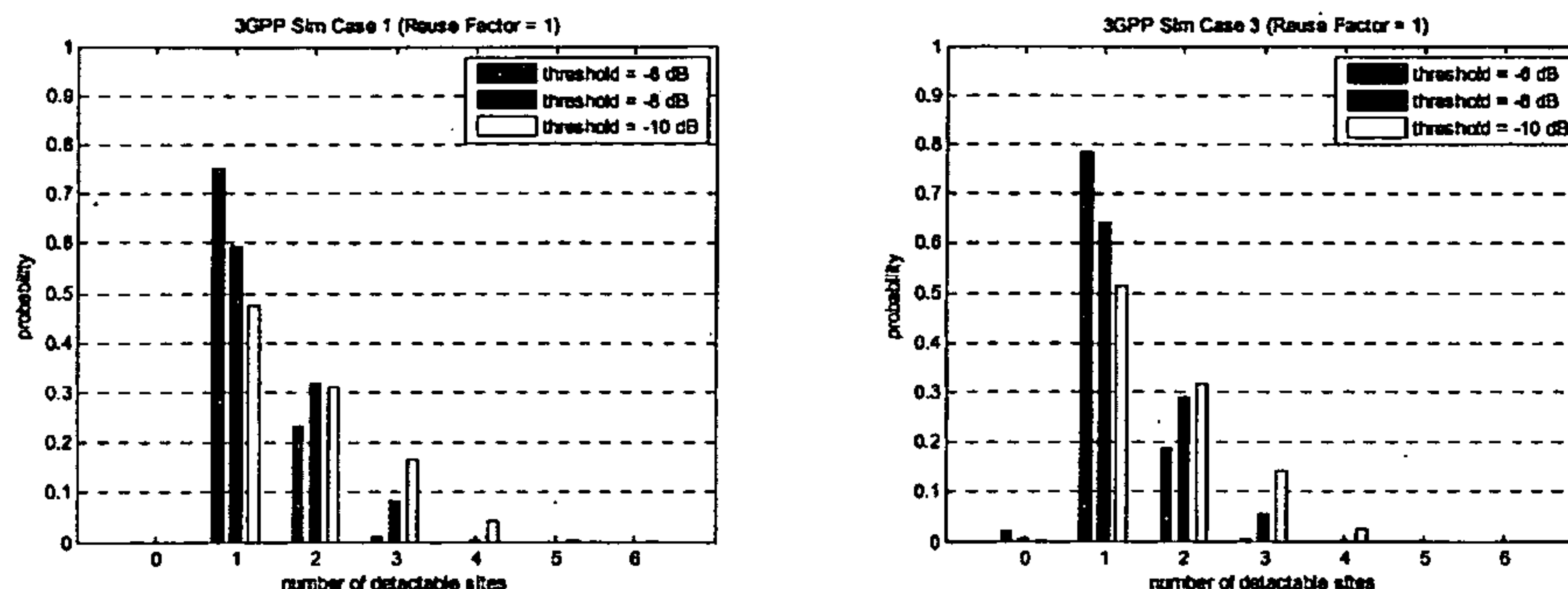
Figure 4: Distributions of number of detectable sites (Reuse Factor = 1).
