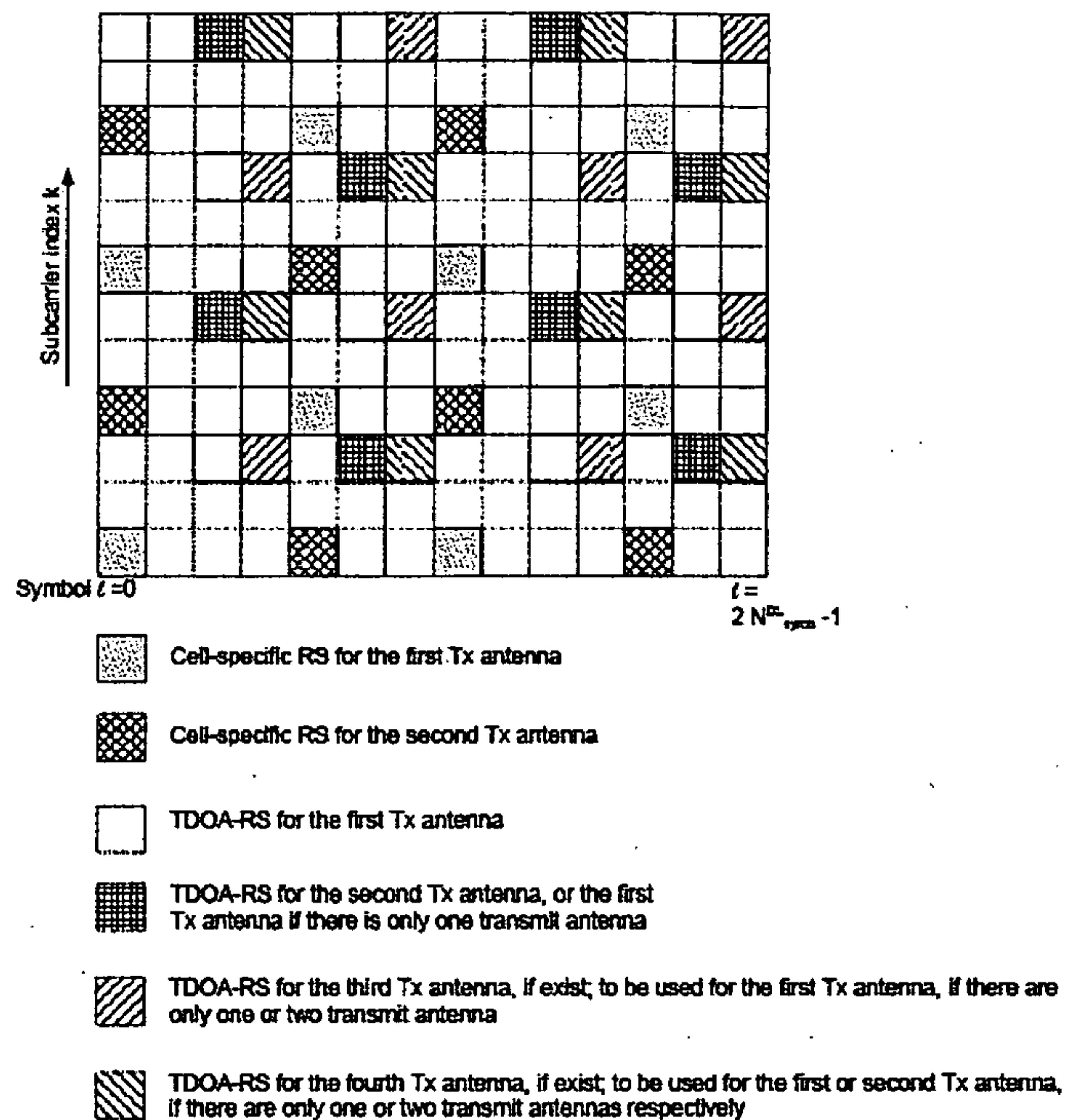
Figure 7 Proposed TDOA-RS structure
