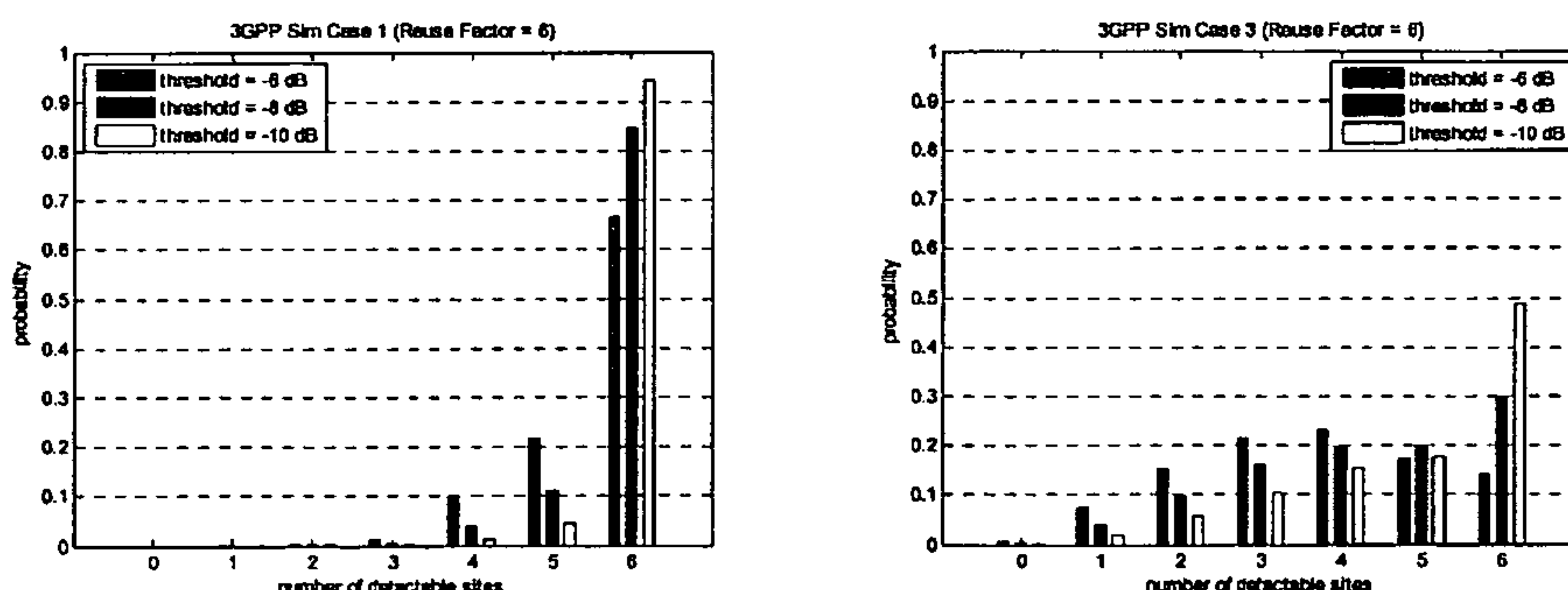
Figure 6: Distributions of number of detectable sites (Reuse Factor = 6).
