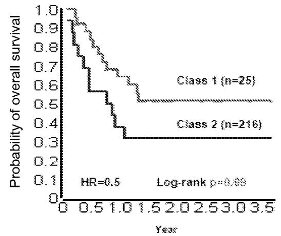
GSE11117 dataset
