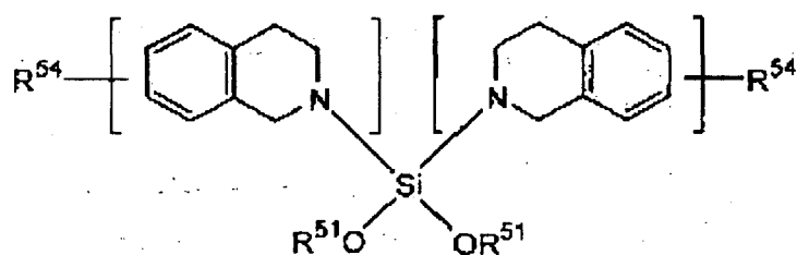
bis(1,2,3,4-tetrahydroisoquinolino) compound
