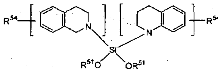
(1,2,3,4-tetrahydroquinolino)(1,2,3,4-tetrahydroisoquinolino) compound
