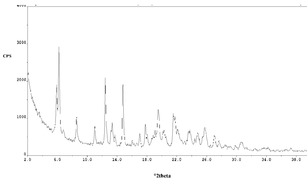
Figure 1: X-ray powder diffraction pattern (XRPD) of Mitapivat hemisulfate Form M1
