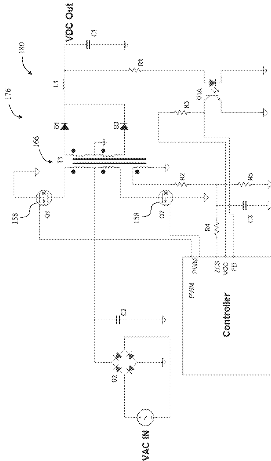
Asynchronous Modified Push-Pull Converter
