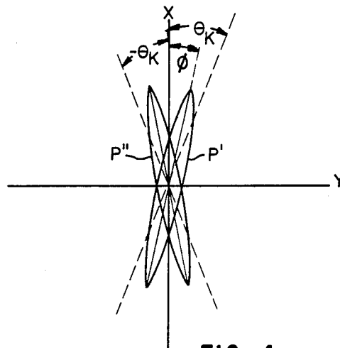
FIG. 4 (PRIOR ART)
