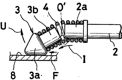
Fig. 3 (PRIOR ART)
