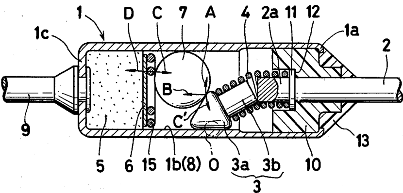
Fig. 1 (PRIOR ART)
