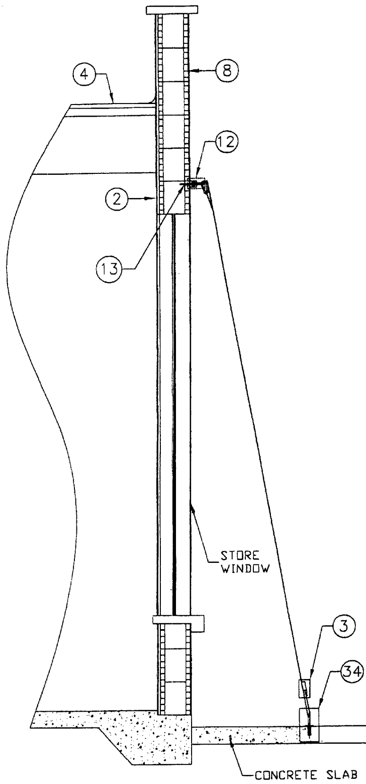
FIGURE 1 - SECTION @ WALL
