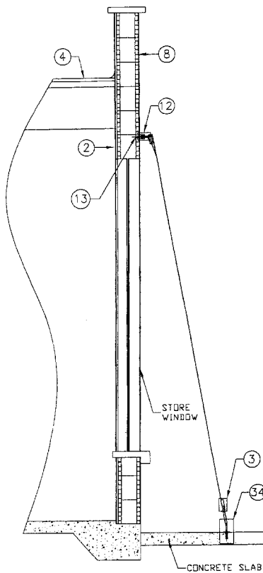
SECTION @ WALL
