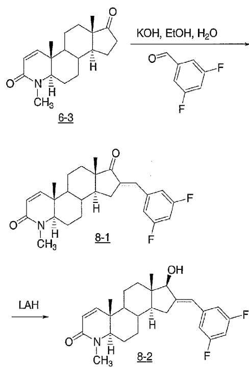
SCHEME 8
