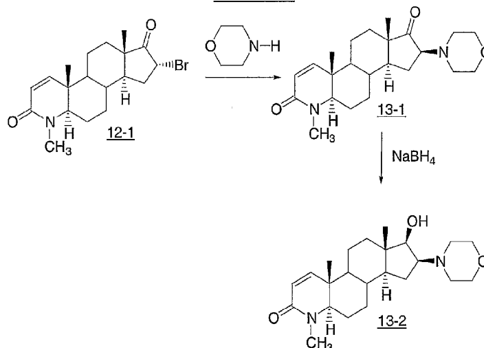
SCHEME 13
