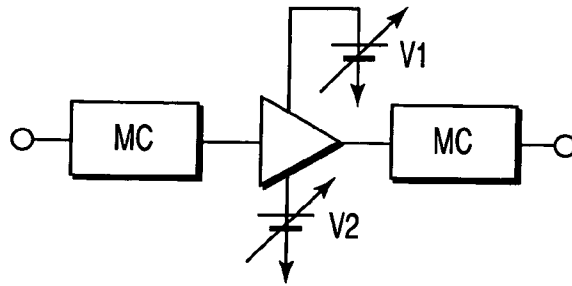
FIG. 14 PRIOR ART
