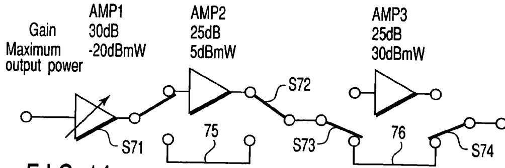
FIG. 14 PRIOR ART
