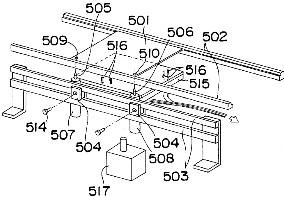
Fig. 19 PRIOR ART
