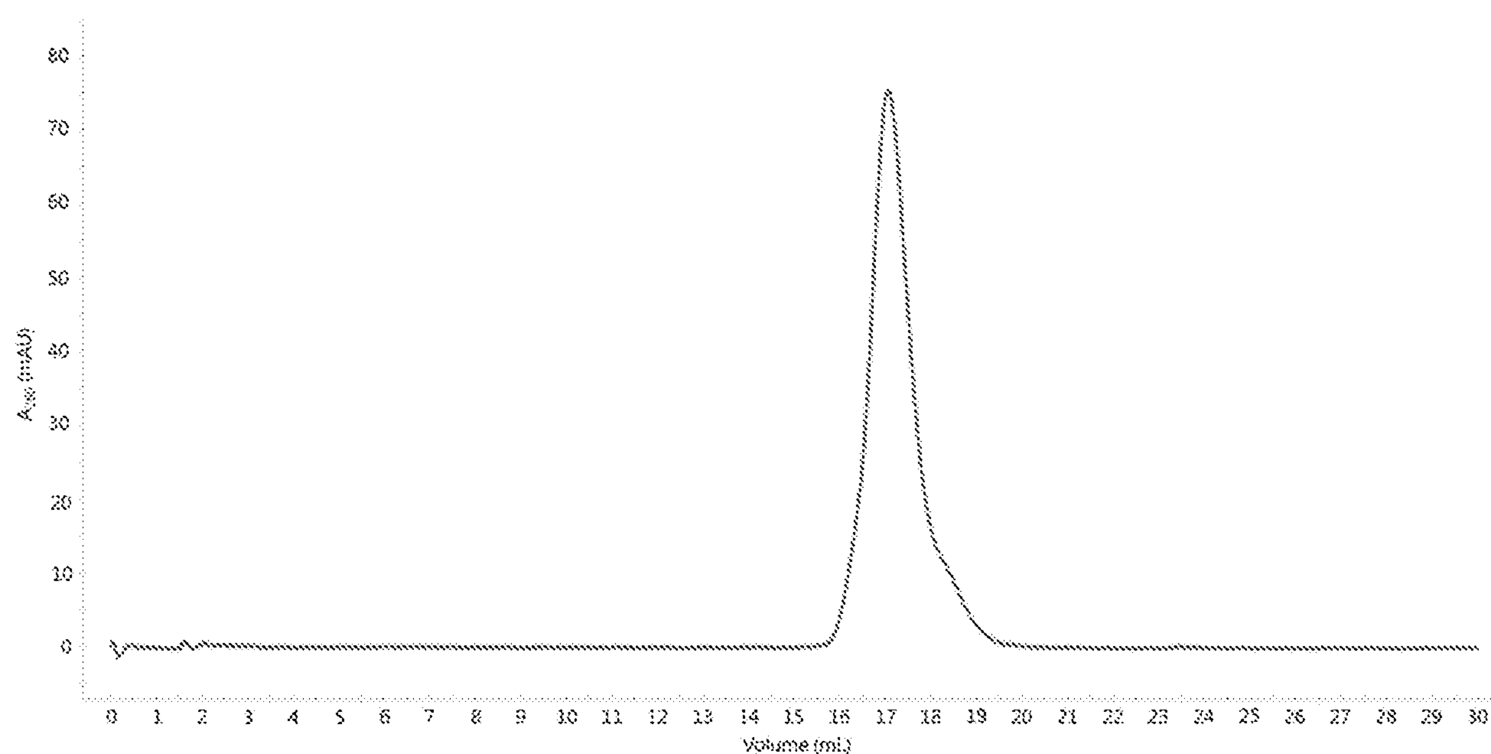
Size exclusion chromatogram of multispecific molecule 8
