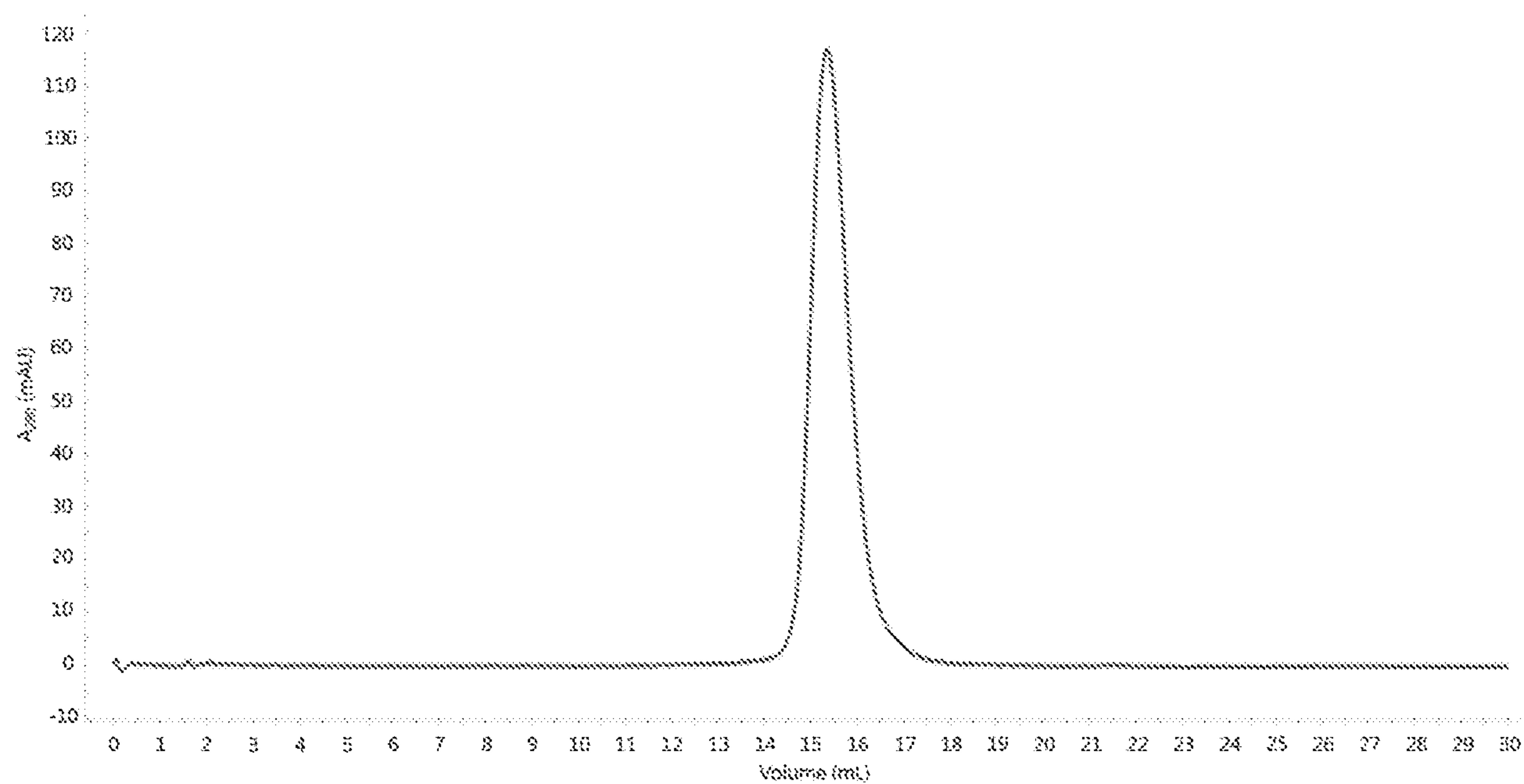
Size exclusion chromatogram of multispecific molecule 9
