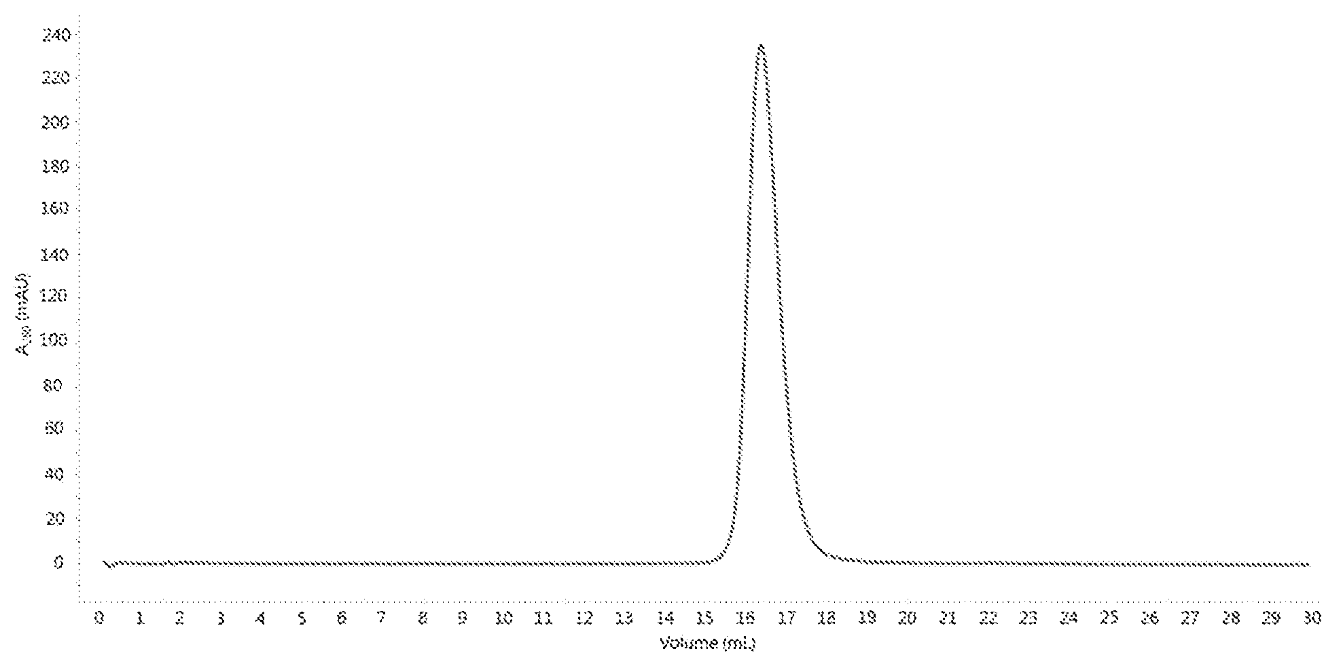
Size exclusion chromatogram of multispecific molecule 3
