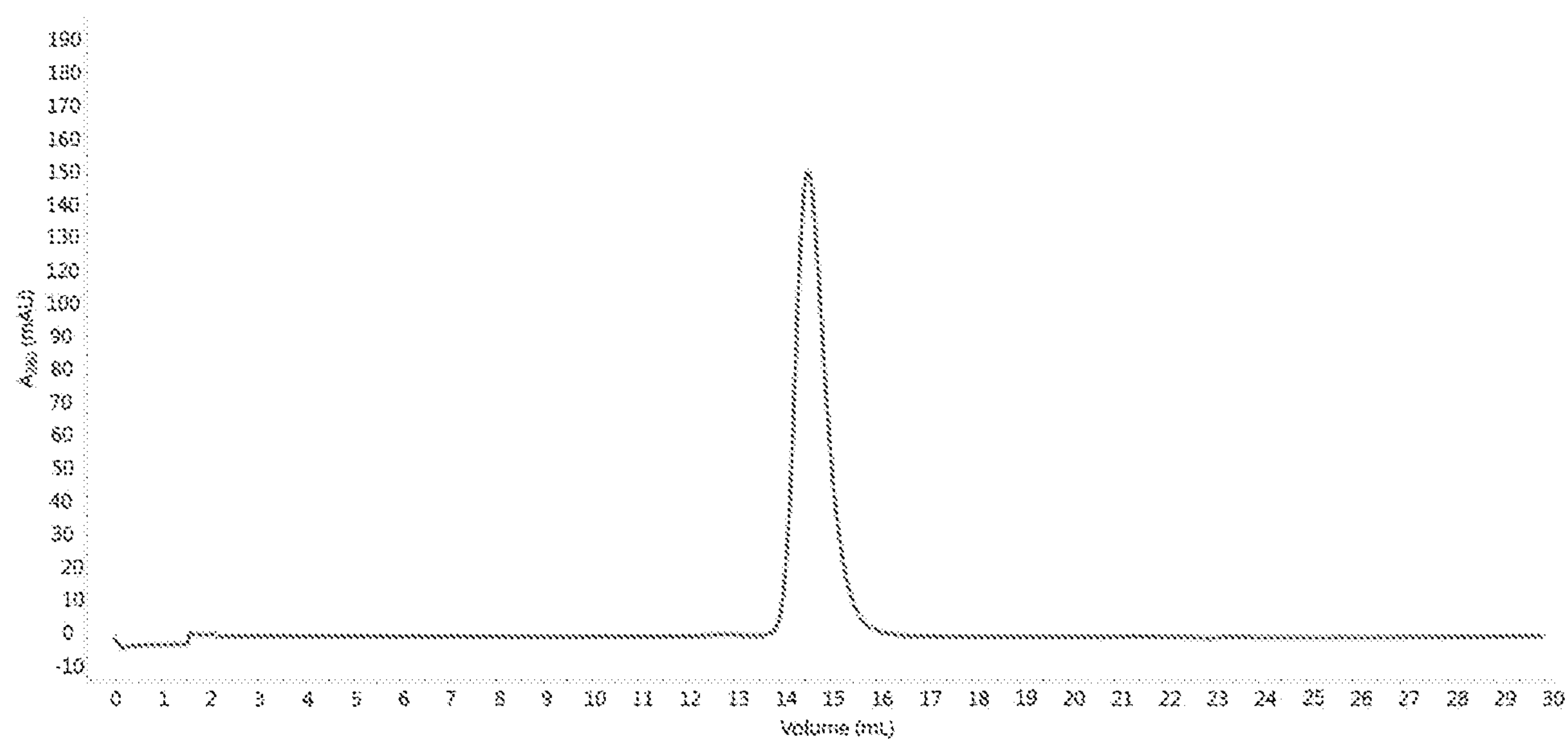
Size exclusion chromatogram of multispecific molecule 1
