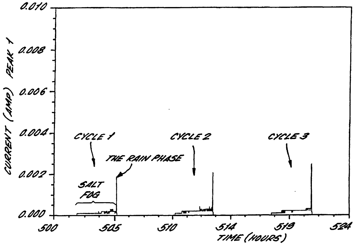
FIG. 5a. LEAKAGE CURRENT WITH INSULATORS
