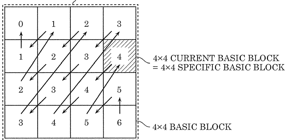
FIG. 21 THE NUMBER OF NON-ZERO COEFFICIENTS IN PRECEDING BASIC BLOCK
