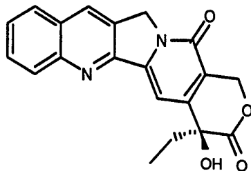
(S)-Camptothecin
