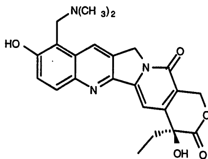
(S)-Topotecan
