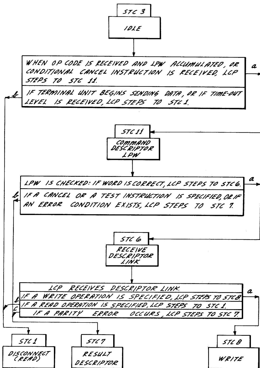
FIG. 7A SIMPLIFIED RECEIPT-OF-INSTRUCTIONS FLOW
