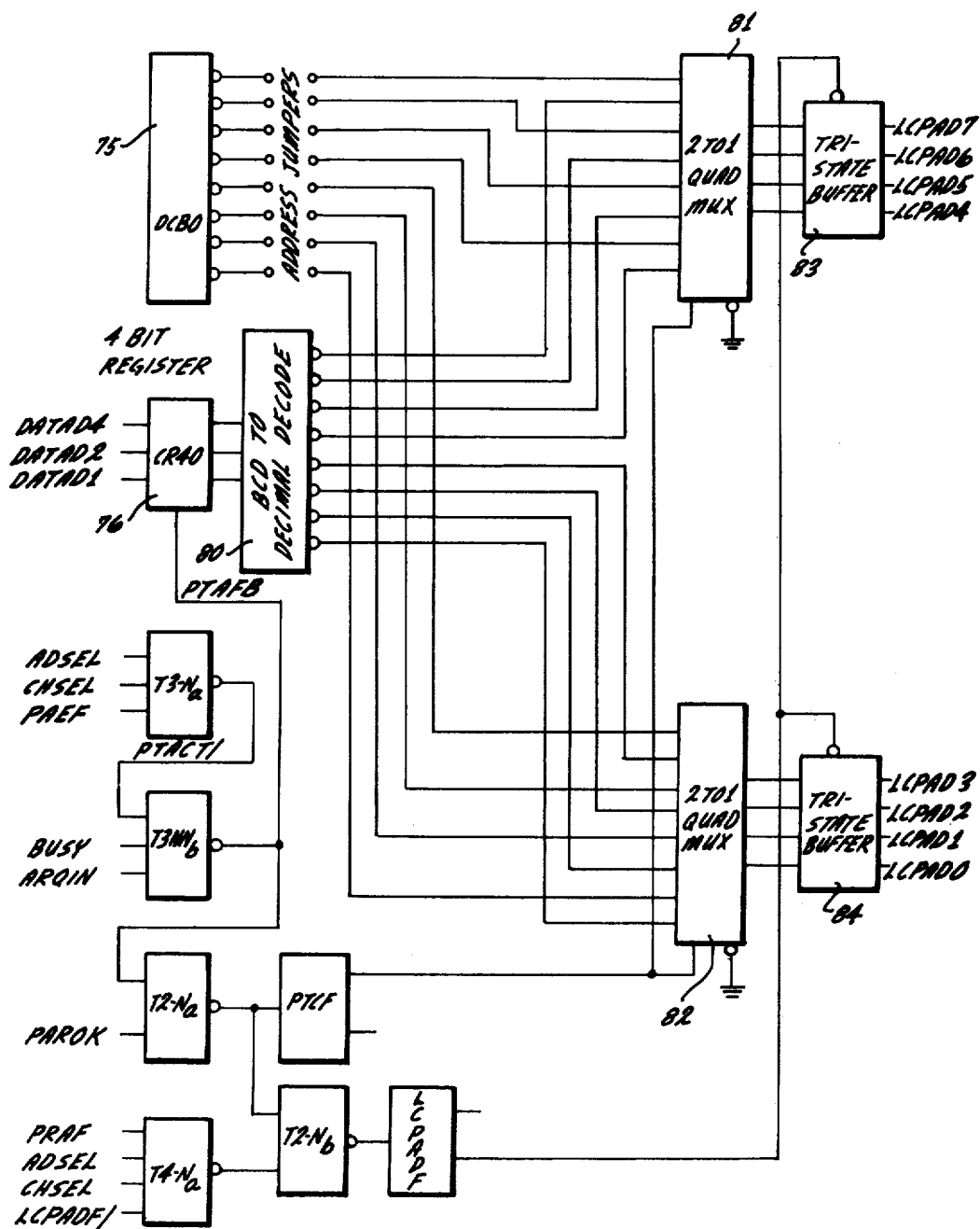
Fig. 5c-20a DISTRIBUTION CARD (LLP ADDRESS DECODING)
