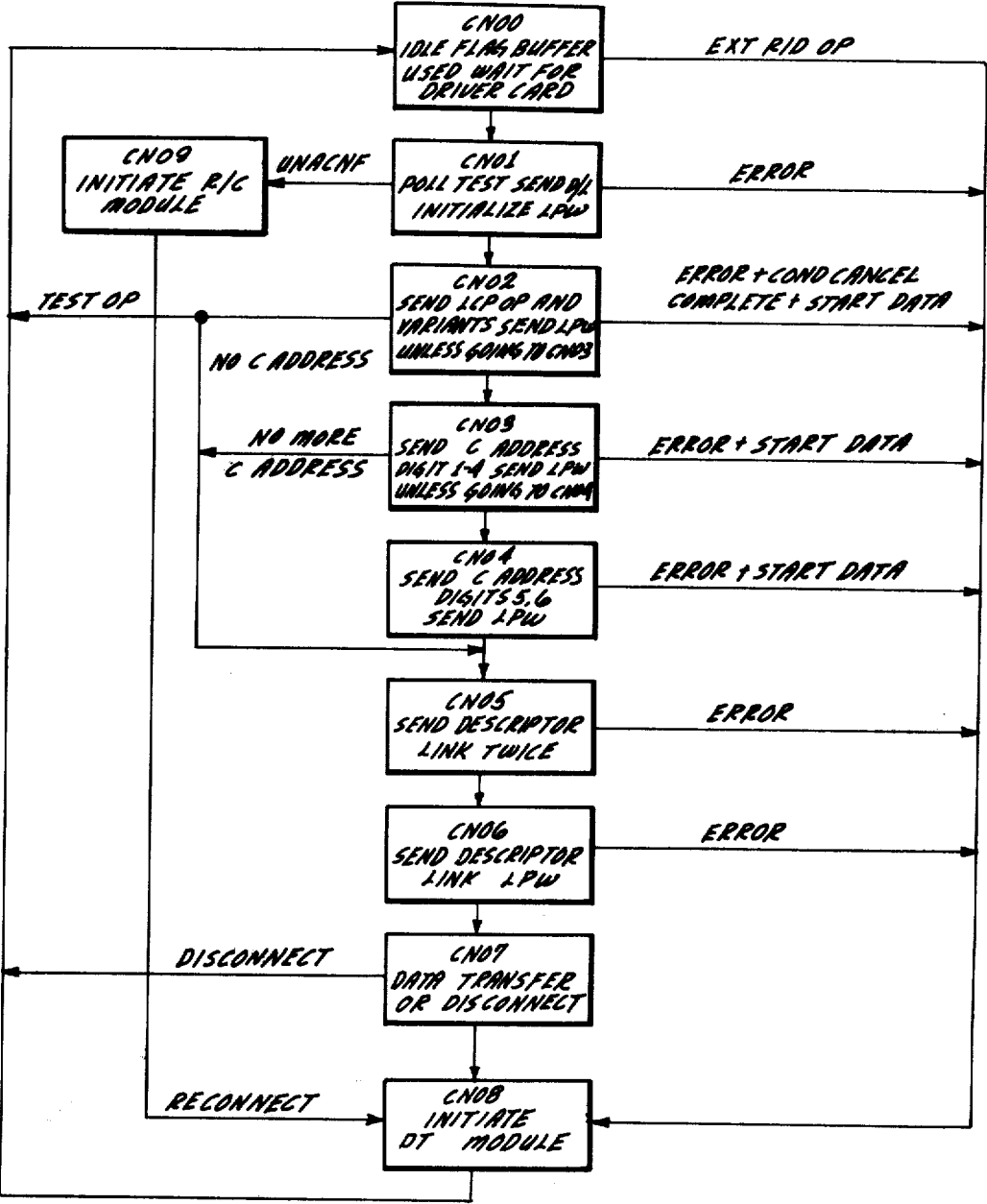
Fig. 5C-18 CONNECTION MODULE FLOW
