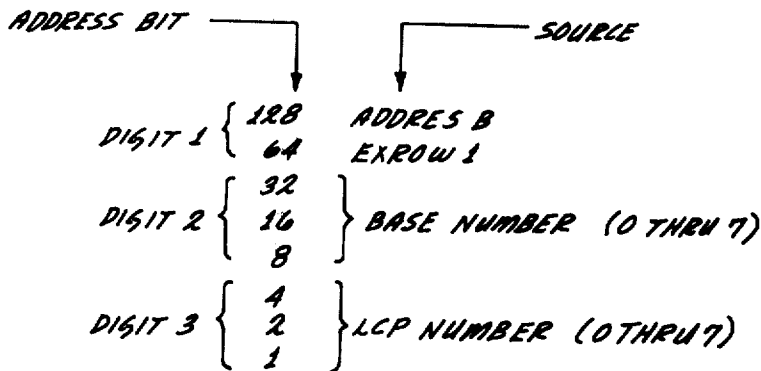
FIG. 5F IOT SCRATCHPAD MEMORY
