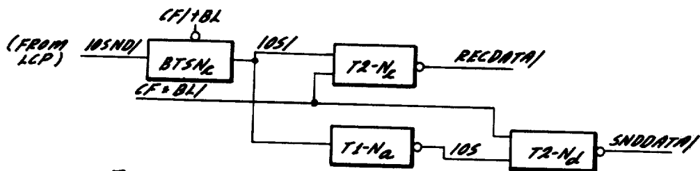
Fig. 5C-22 WRITE CYCLE DATA TRANSFERS
