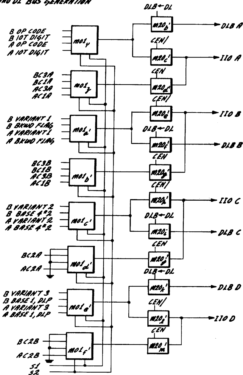
Fig. 51-19 IIO AND DL BUS GENERATION
