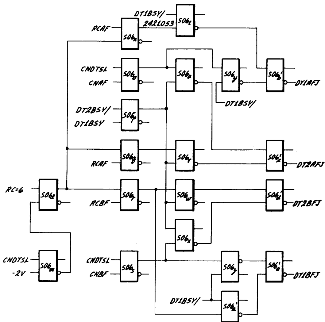
FIG. 56-12 DATA TRANSFER MODULE (MODULE SELECT LOGIC)
