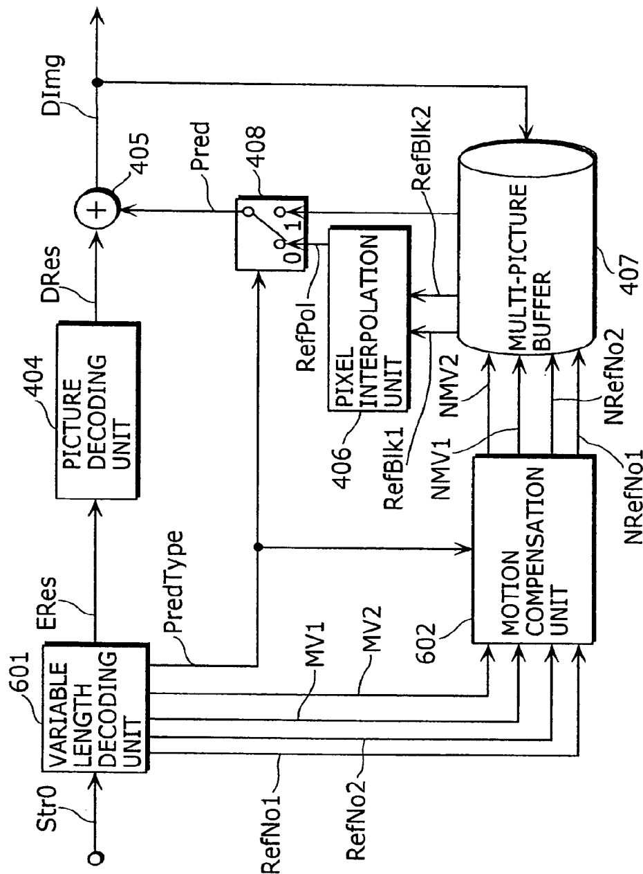
FIG. 4 PRIOR ART
