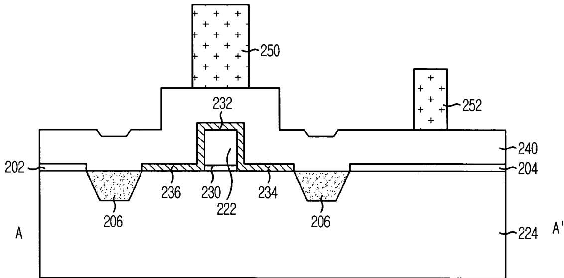
FIG. 2C (PRIOR ART)
