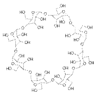
\gamma -cyclodextrin
