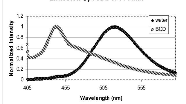
Emission Spectra of Prodan
