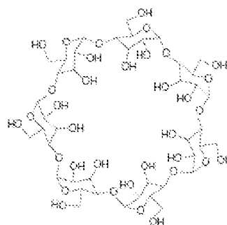
\beta -cyclodextrin
