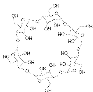
\gamma -cyclodextrin
