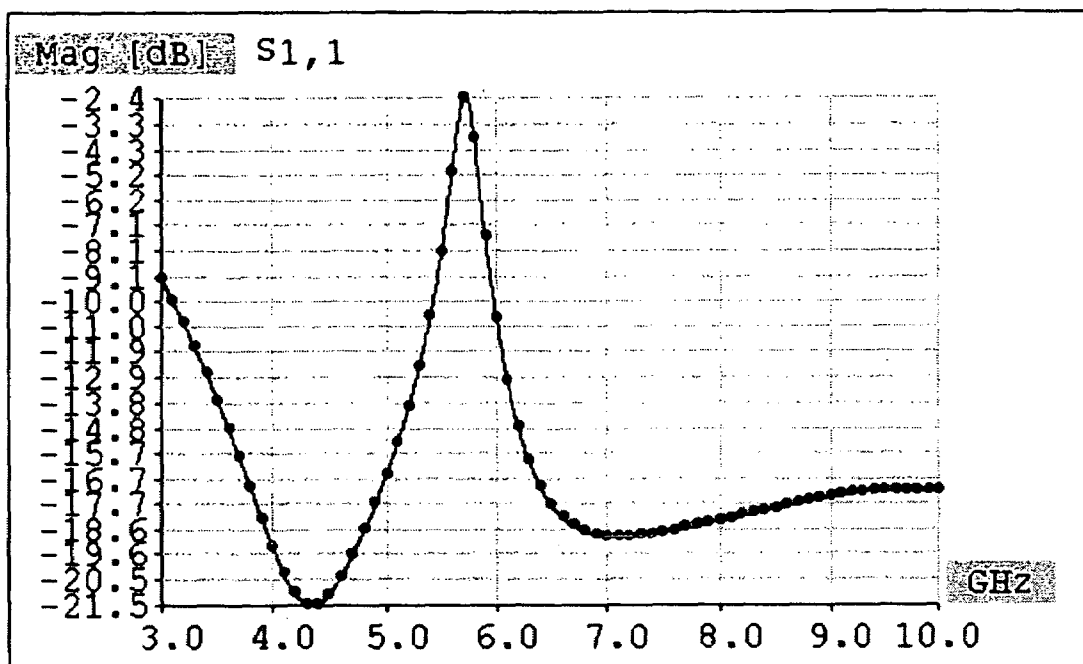
Fig.6: An example of an antenna matching
