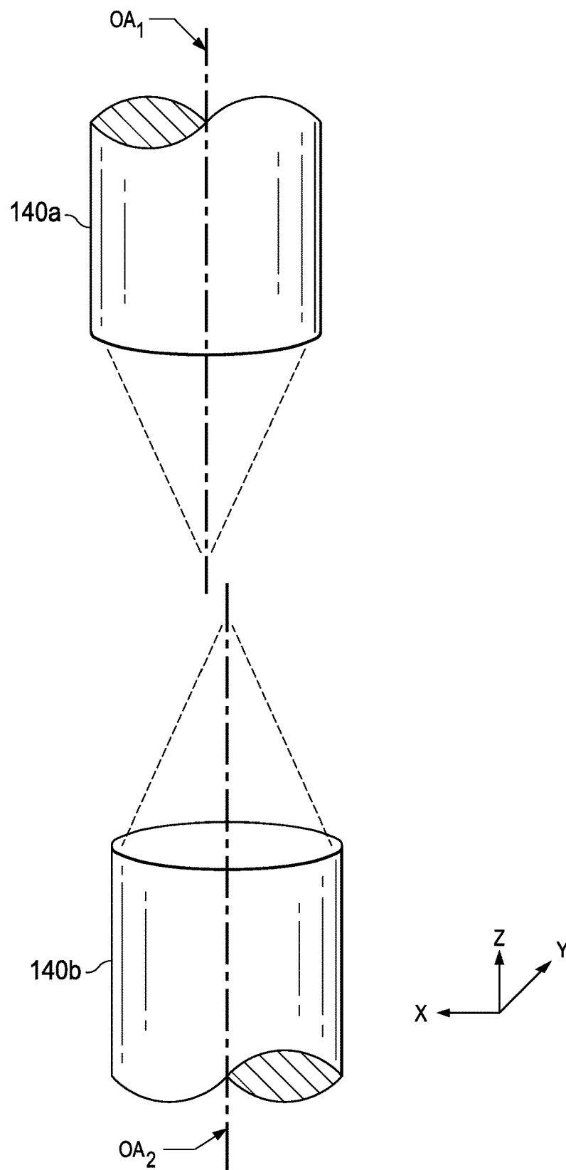
FIG. 1C (PRIOR ART)
