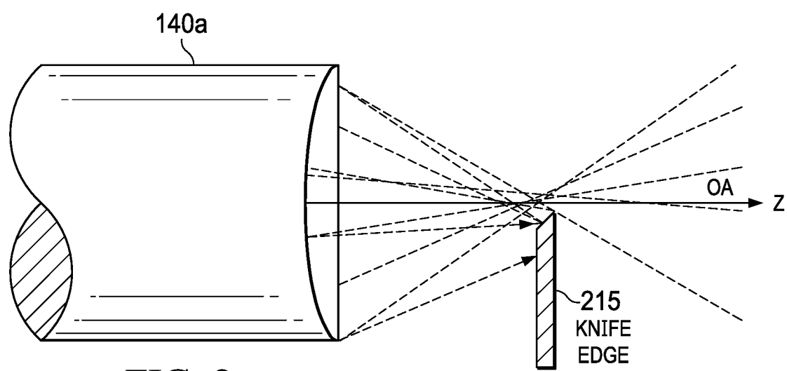
FIG. 2 (PRIOR ART)
